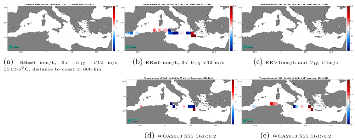
Figure 14: Temporal mean gridded over spatial boxes of size 1^\circ \times 1^\circ of \Delta\text{SSS} (SMOS SSS L3 v332 - 9 Days (CATDS-CPDC) - TSG (SAMOS)) for 5 different subdatasets corresponding to:RR=0 mm/h, 3 < U_{10} < 12 m/s, SST > 5°C, distance to coast > 800 km (a), RR=0 mm/h, 3 < U_{10} < 12 m/s (b), RR > 1mm/h and U_{10} < 4 m/s (c), WOA2013 SSS Std < 0.2 (d), WOA2013 SSS Std > 0.2 (e).
