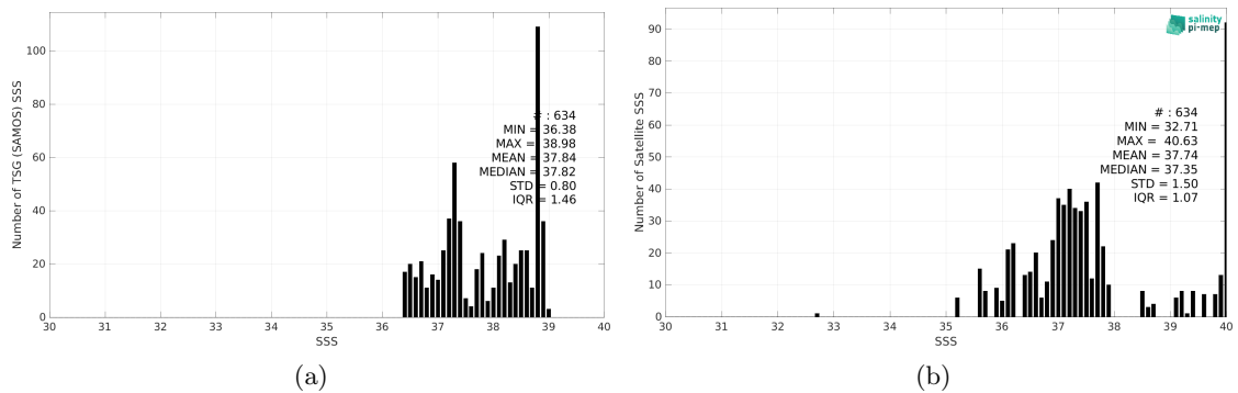
Figure 2: Histograms of SSS from TSG (SAMOS) (a) and SMOS SSS L3 v332 - 9 Days (CATDS-CPDC) (b) considering all match-up pairs per bins of 0.1 over the Mediterranean Sea Pi-MEP region and for the full satellite product period.
