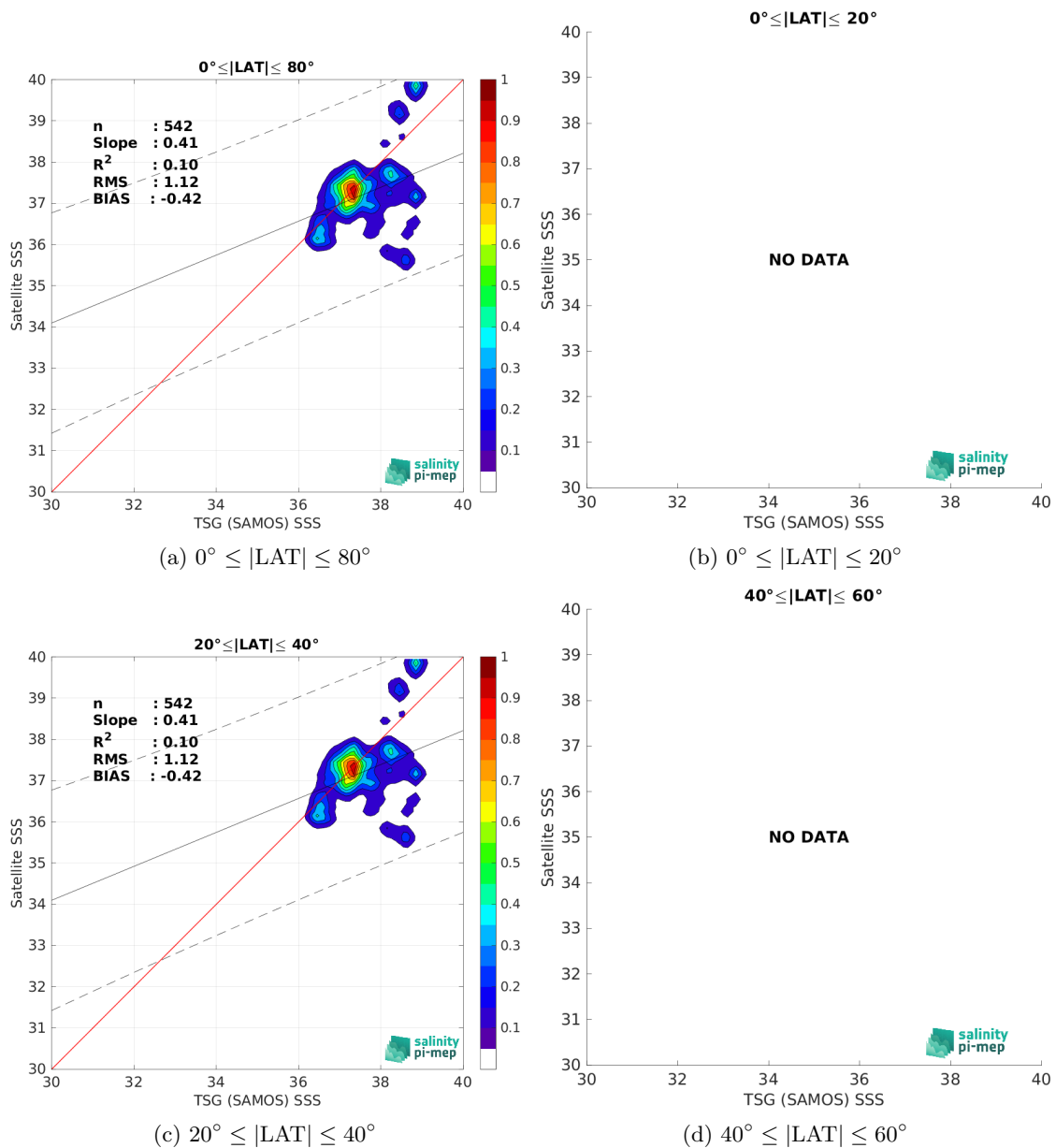
Figure 9: Contour maps of the concentration of SMOS SSS L3 v332 - 9 Days (CATDS-CPDC) SSS (y-axis) versus TSG (SAMOS) SSS (x-axis) at match-up pairs for different latitude bands. For each plot, the red line shows x=y . The black thin and dashed lines indicate a linear fit through the data cloud and the \pm 95\% confidence levels, respectively. The number match-up pairs n , the slope and R^2 coefficient of the linear fit, the root mean square (RMS) and the mean bias between satellite and in situ data are indicated for each latitude band in each plots.
