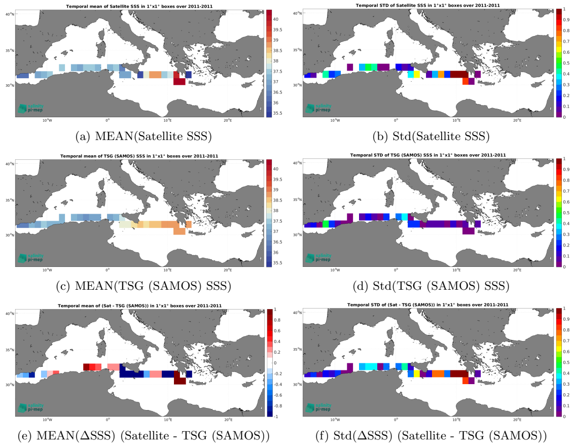
Figure 6: Temporal mean (left) and Std (right) of SSS from SMOS SSS L3 v332 - 9 Days (CATDS-CPDC) (top), TSG (SAMOS) (middle), and of \Delta SSS (Satellite - TSG (SAMOS)). Only match-up pairs are used to generate these maps.
