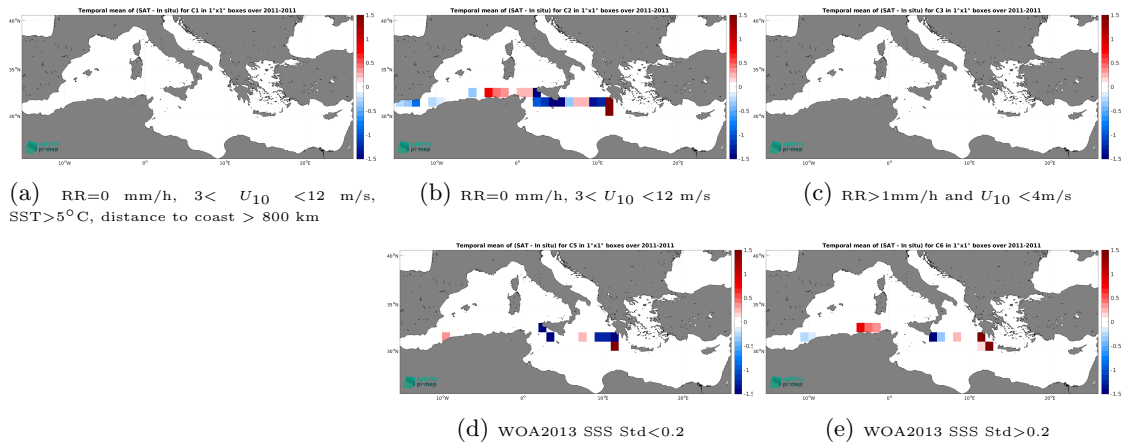
Figure 12: Temporal mean gridded over spatial boxes of size 1^{\circ}\times 1^{\circ} of \Delta\text{SSS} (SMOS SSS L3 v332 - 9 Days (CATDS-CPDC) - TSG (SAMOS)) for 5 different subdatasets corresponding to:RR=0 mm/h, 3 < U_{10} < 12 m/s, SST >5^{\circ}\text{C} , distance to coast > 800 km (a), RR=0 mm/h, 3 < U_{10} < 12 m/s (b), RR >1 mm/h and U_{10} < 4 m/s (c), WOA2013 SSS Std <0.2 (d), WOA2013 SSS Std >0.2 (e).
