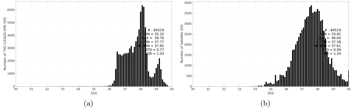
Figure 3: Histograms of SSS from TSG (LEGOS-DM) (a) and SMOS SSS L3 v332 - 9 Days (CATDS-CPDC) (b) considering all match-up pairs per bins of 0.1 over the Mediterranean Sea Pi-MEP region and for the full satellite product period.
