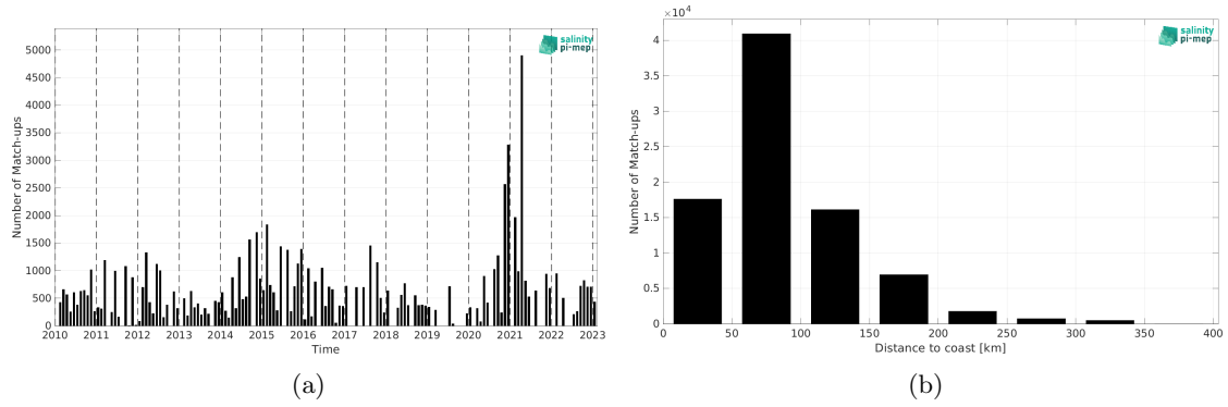
Figure 2: Number of match-ups between TSG (LEGOS-DM) and SMOS SSS L3 v332 - 9 Days (CATDS-CPDC) SSS as a function of time (a) and as function of the distance to coast (b) over the Mediterranean Sea Pi-MEP region and for the full satellite product period.
