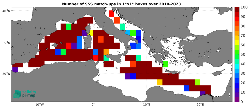
Figure 5: Number of SSS match-ups between TSG (LEGOS-DM) SSS and the SMOS SSS L3 v332 - 9 Days (CATDS-CPDC) SSS product for the Mediterranean Sea Pi-MEP region over 1^\circ \times 1^\circ boxes and for the full satellite product period.
