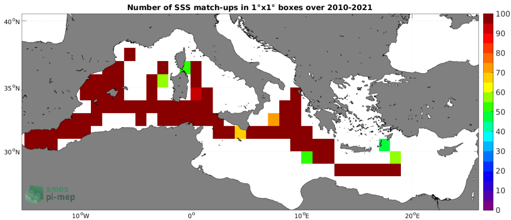
Figure 4: Number of SSS match-ups between TSG (CSIC-UTM) SSS and the SMOS SSS L3 v332 - 9 Days (CATDS-CPDC) SSS product for the Mediterranean Sea Pi-MEP region over 1^\circ \times 1^\circ boxes and for the full satellite product period.
