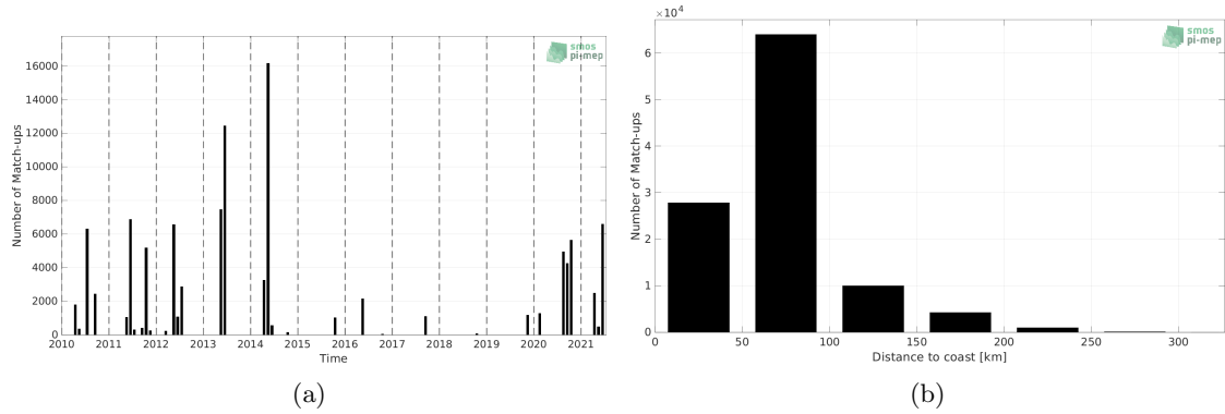
Figure 1: Number of match-ups between TSG (CSIC-UTM) and SMOS SSS L3 v332 - 9 Days (CATDS-CPDC) SSS as a function of time (a) and as function of the distance to coast (b) over the Mediterranean Sea Pi-MEP region and for the full satellite product period.
