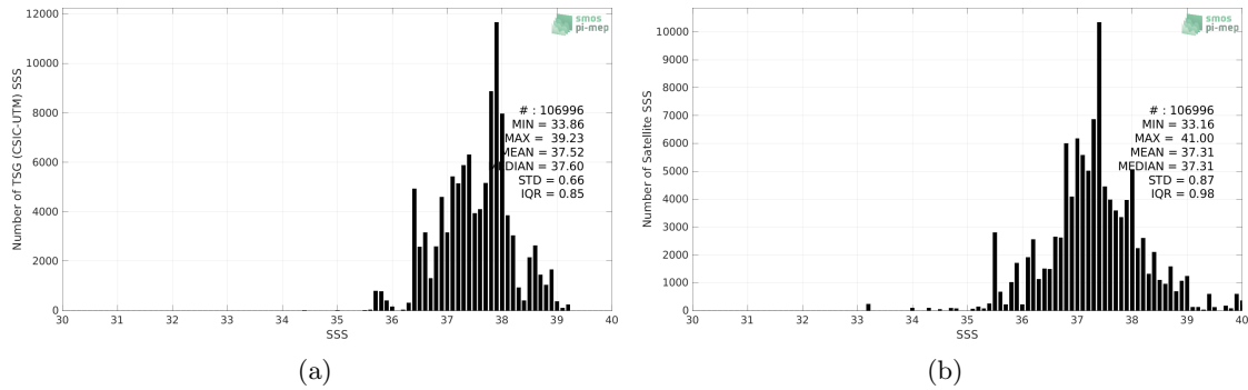
Figure 2: Histograms of SSS from TSG (CSIC-UTM) (a) and SMOS SSS L3 v332 - 9 Days (CATDS-CPDC) (b) considering all match-up pairs per bins of 0.1 over the Mediterranean Sea Pi-MEP region and for the full satellite product period.
