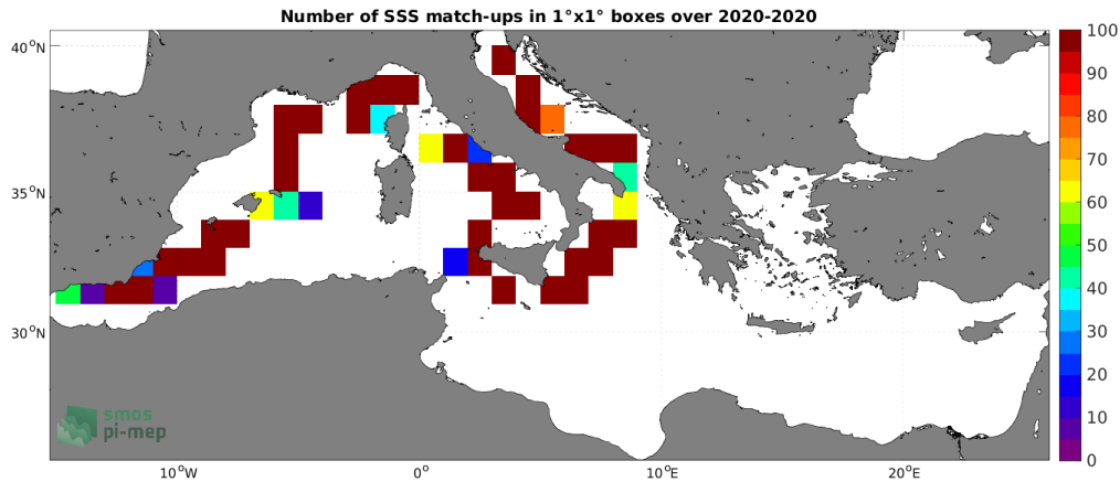
Figure 4: Number of SSS match-ups between Saildrone SSS and the SMOS SSS L3 v332 - 9 Days (CATDS-CPDC) SSS product for the Mediterranean Sea Pi-MEP region over 1^\circ \times 1^\circ boxes and for the full satellite product period.
