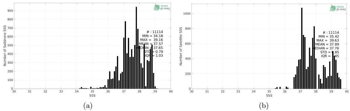
Figure 2: Histograms of SSS from Saildrone (a) and SMOS SSS L3 v332 - 9 Days (CATDS-CPDC) (b) considering all match-up pairs per bins of 0.1 over the Mediterranean Sea Pi-MEP region and for the full satellite product period.
