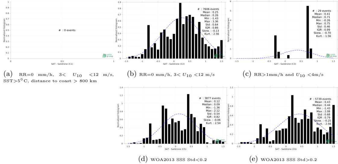
Figure 13: Normalized histogram of \Delta\text{SSS} (SMOS SSS L3 v332 - 9 Days (CATDS-CPDC) - Saildrone) for 5 different subdatasets corresponding to: RR=0 mm/h, 3 < U_{10} < 12 m/s, SST > 5^{\circ}\text{C} , distance to coast > 800 km (a), RR=0 mm/h, 3 < U_{10} < 12 m/s (b), RR > 1\text{mm/h} and U_{10} < 4\text{m/s} (c), WOA2013 SSS Std < 0.2 (d), WOA2013 SSS Std > 0.2 (e).
