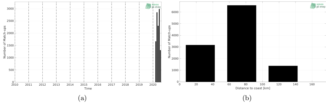
Figure 1: Number of match-ups between Saildrone and SMOS SSS L3 v332 - 9 Days (CATDS-CPDC) SSS as a function of time (a) and as function of the distance to coast (b) over the Mediterranean Sea Pi-MEP region and for the full satellite product period.
