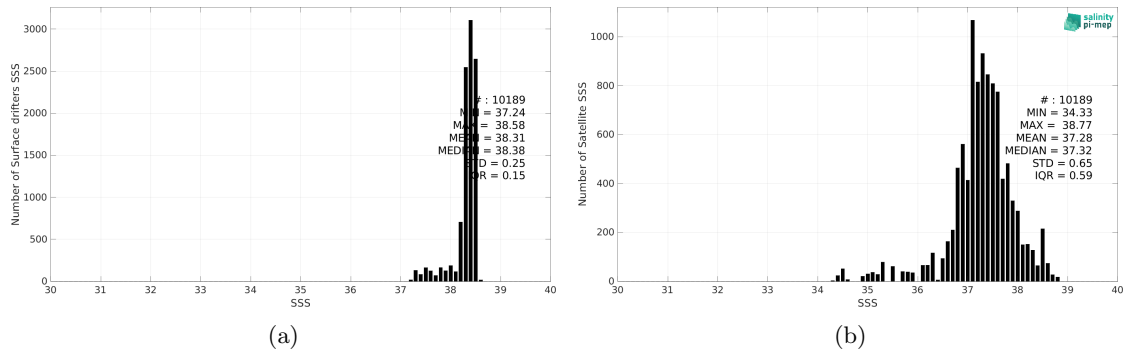
Figure 2: Histograms of SSS from Surface drifters (a) and SMOS SSS L3 v332 - 9 Days (CATDS-CPDC) (b) considering all match-up pairs per bins of 0.1 over the Mediterranean Sea Pi-MEP region and for the full satellite product period.
