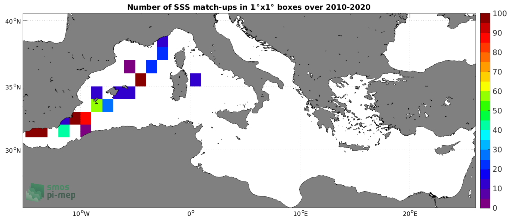
Figure 4: Number of SSS match-ups between TSG (LEGOS-DM) SSS and the SMOS SSS L2Q v331 - 0.25 Deg (CATDS-CPDC) SSS product for the Mediterranean Sea Pi-MEP region over 1^\circ \times 1^\circ boxes and for the full satellite product period.
