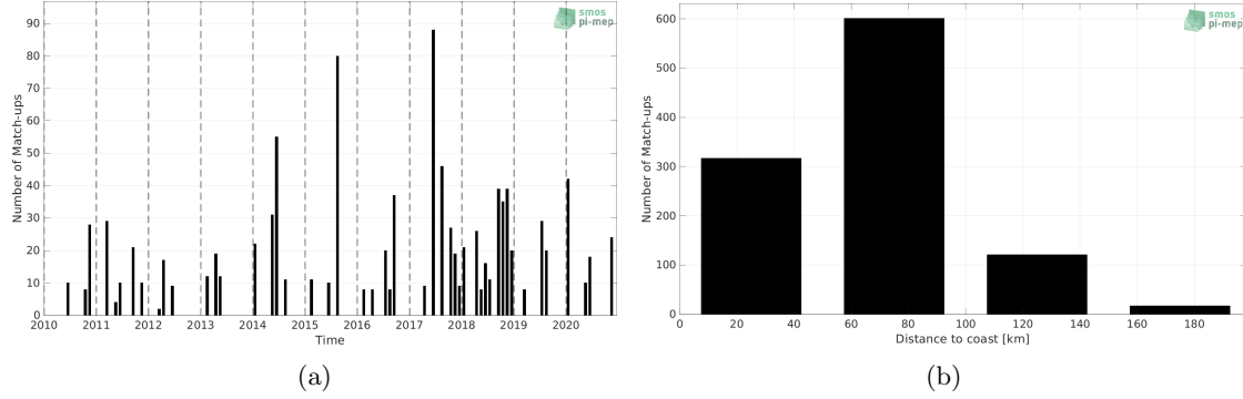
Figure 1: Number of match-ups between TSG (LEGOS-DM) and SMOS SSS L2Q v331 - 0.25 Deg (CATDS-CPDC) SSS as a function of time (a) and as function of the distance to coast (b) over the Mediterranean Sea Pi-MEP region and for the full satellite product period.
