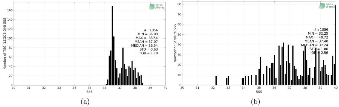
Figure 2: Histograms of SSS from TSG (LEGOS-DM) (a) and SMOS SSS L2Q v331 - 0.25 Deg (CATDS-CPDC) (b) considering all match-up pairs per bins of 0.1 over the Mediterranean Sea Pi-MEP region and for the full satellite product period.
