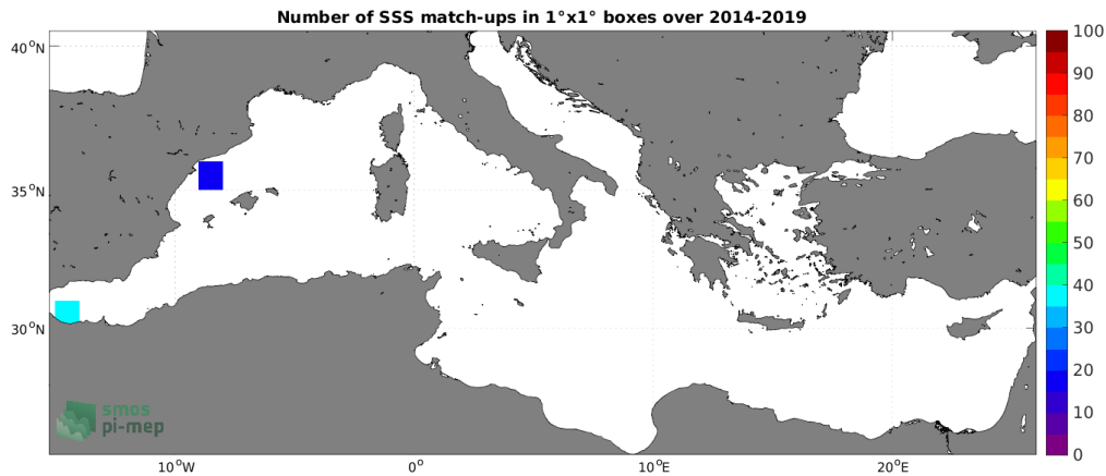
Figure 4: Number of SSS match-ups between TSG (GOSUD-Sailing-ship) SSS and the SMOS SSS L2Q v331 - 0.25 Deg (CATDS-CPDC) SSS product for the Mediterranean Sea Pi-MEP region over 1^\circ \times 1^\circ boxes and for the full satellite product period.
