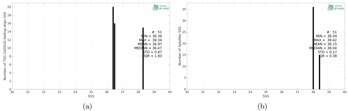
Figure 2: Histograms of SSS from TSG (GOSUD-Sailing-ship) (a) and SMOS SSS L2Q v331 - 0.25 Deg (CATDS-CPDC) (b) considering all match-up pairs per bins of 0.1 over the Mediterranean Sea Pi-MEP region and for the full satellite product period.
