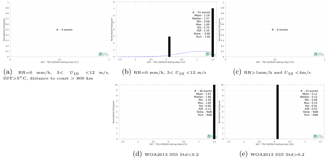
Figure 13: Normalized histogram of \Delta\text{SSS} (SMOS SSS L2Q v331 - 0.25 Deg (CATDS-CPDC) - TSG (GOSUD-Sailing-ship)) for 5 different subdatasets corresponding to: RR=0 mm/h, 3 < U_{10} < 12 m/s, SST > 5^{\circ}\text{C} , distance to coast > 800 km (a), RR=0 mm/h, 3 < U_{10} < 12 m/s (b), RR > 1\text{mm/h} and U_{10} < 4\text{m/s} (c), WOA2013 SSS Std < 0.2 (d), WOA2013 SSS Std > 0.2 (e).
