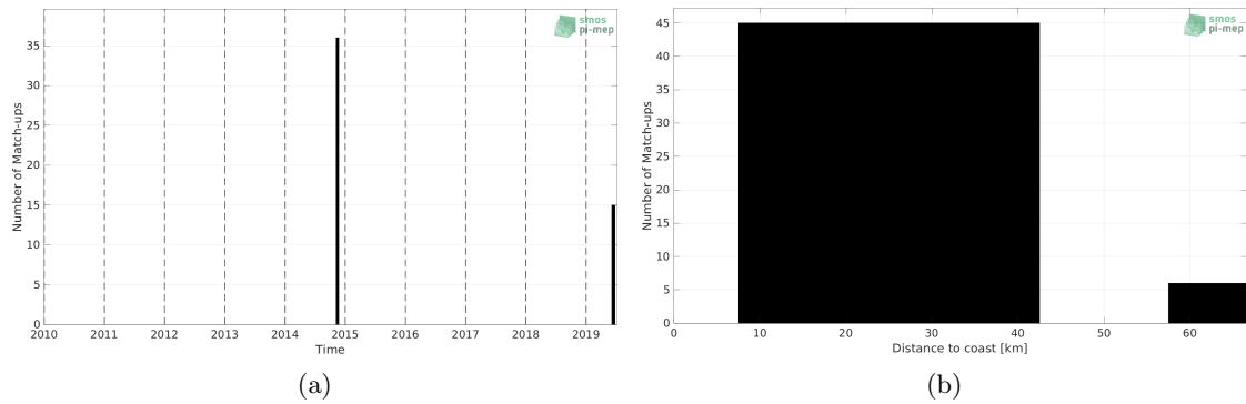
Figure 1: Number of match-ups between TSG (GOSUD-Sailing-ship) and SMOS SSS L2Q v331 - 0.25 Deg (CATDS-CPDC) SSS as a function of time (a) and as function of the distance to coast (b) over the Mediterranean Sea Pi-MEP region and for the full satellite product period.
