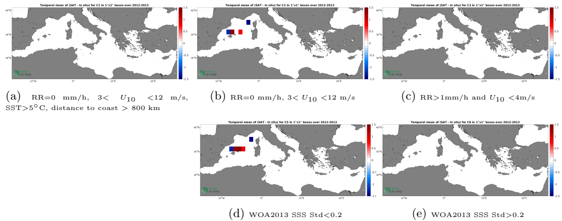
Figure 11: Temporal mean gridded over spatial boxes of size 1^{\circ}\times 1^{\circ} of \Delta\text{SSS} (SMOS SSS L2Q v331 - 0.25 Deg (CATDS-CPDC) - Surface drifters) for 5 different subdatasets corresponding to:RR=0 mm/h, 3 < U_{10} < 12 m/s, SST >5^{\circ}\text{C} , distance to coast > 800 km (a), RR=0 mm/h, 3 < U_{10} < 12 m/s (b), RR >1 mm/h and U_{10} < 4 m/s (c), WOA2013 SSS Std <0.2 (d), WOA2013 SSS Std >0.2 (e).
