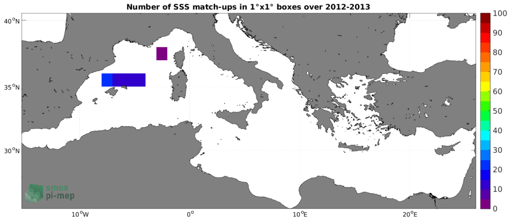
Figure 3: Number of SSS match-ups between Surface drifters SSS and the SMOS SSS L2Q v331 - 0.25 Deg (CATDS-CPDC) SSS product for the Mediterranean Sea Pi-MEP region over 1^\circ \times 1^\circ boxes and for the full satellite product period.
