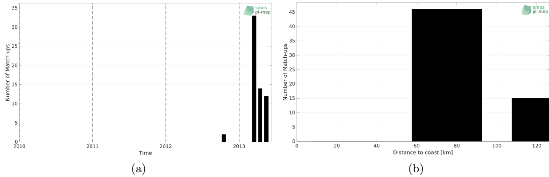
Figure 1: Number of match-ups between Surface drifters and SMOS SSS L2Q v331 - 0.25 Deg (CATDS-CPDC) SSS as a function of time (a) and as function of the distance to coast (b) over the Mediterranean Sea Pi-MEP region and for the full satellite product period.
