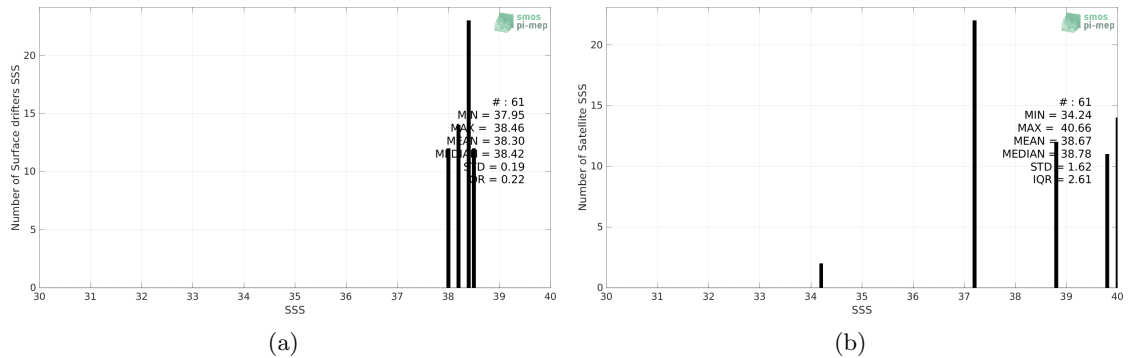
Figure 2: Histograms of SSS from Surface drifters (a) and SMOS SSS L2Q v331 - 0.25 Deg (CATDS-CPDC) (b) considering all match-up pairs per bins of 0.1 over the Mediterranean Sea Pi-MEP region and for the full satellite product period.
