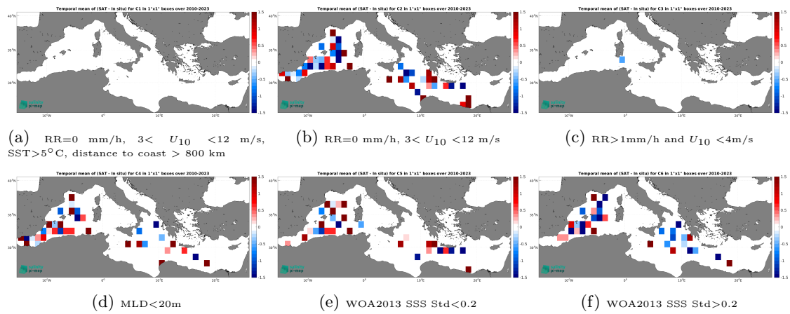
Figure 12: Temporal mean gridded over spatial boxes of size 1^\circ \times 1^\circ of \Delta SSS (SMOS SSS L2Q v331 - 0.25 Deg (CATDS-CPDC) - Argo) for 6 different subdatasets corresponding to:RR=0 mm/h, 3 < U_{10} < 12 m/s, SST >5^\circ C, distance to coast > 800 km (a), RR=0 mm/h, 3 < U_{10} < 12 m/s (b), RR >1 mm/h and U_{10} < 4 m/s (c),MLD <20 m (d),WOA2013 SSS Std <0.2 (e),WOA2013 SSS Std >0.2 (f).
