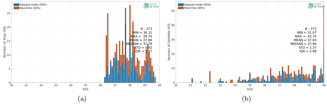
Figure 2: Histograms of SSS from Argo (a) and SMOS SSS L2Q v331 - 0.25 Deg (CATDS-CPDC) (b) considering all match-up pairs per bins of 0.1 over the Mediterranean Sea Pi-MEP region and for the full satellite product period.
