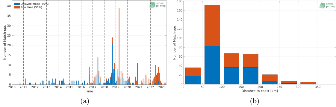
Figure 1: Number of match-ups between Argo and SMOS SSS L2Q v331 - 0.25 Deg (CATDS-CPDC) SSS as a function of time (a) and as function of the distance to coast (b) over the Mediterranean Sea Pi-MEP region and for the full satellite product period.
