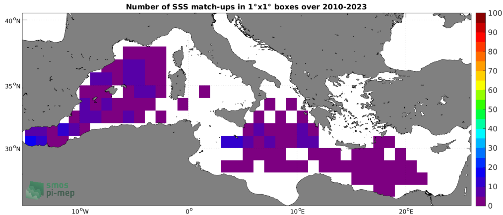
Figure 4: Number of SSS match-ups between Argo SSS and the SMOS SSS L2Q v331 - 0.25 Deg (CATDS-CPDC) SSS product for the Mediterranean Sea Pi-MEP region over 1^\circ \times 1^\circ boxes and for the full satellite product period.
