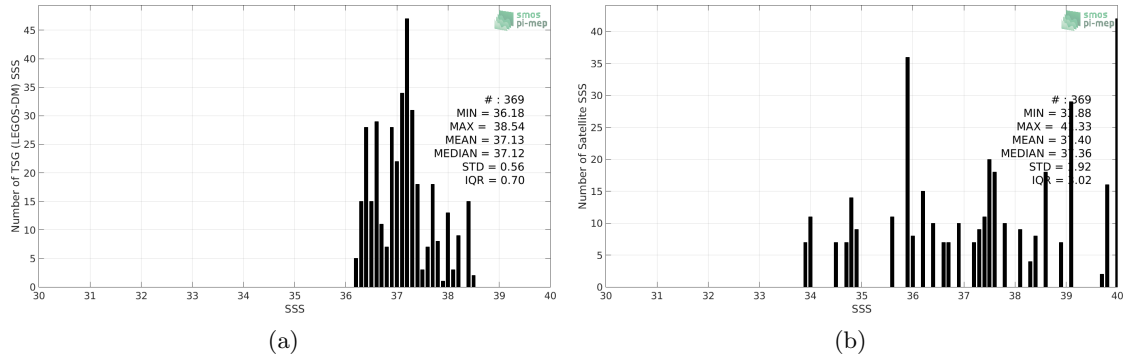
Figure 2: Histograms of SSS from TSG (LEGOS-DM) (a) and SMOS SSS L2Q v321 - 0.25 Deg (CATDS-CPDC) (b) considering all match-up pairs per bins of 0.1 over the Mediterranean Sea Pi-MEP region and for the full satellite product period.
