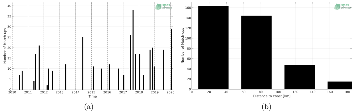
Figure 1: Number of match-ups between TSG (LEGOS-DM) and SMOS SSS L2Q v321 - 0.25 Deg (CATDS-CPDC) SSS as a function of time (a) and as function of the distance to coast (b) over the Mediterranean Sea Pi-MEP region and for the full satellite product period.
