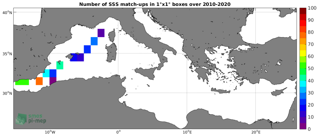
Figure 4: Number of SSS match-ups between TSG (LEGOS-DM) SSS and the SMOS SSS L2Q v321 - 0.25 Deg (CATDS-CPDC) SSS product for the Mediterranean Sea Pi-MEP region over 1^\circ \times 1^\circ boxes and for the full satellite product period.
