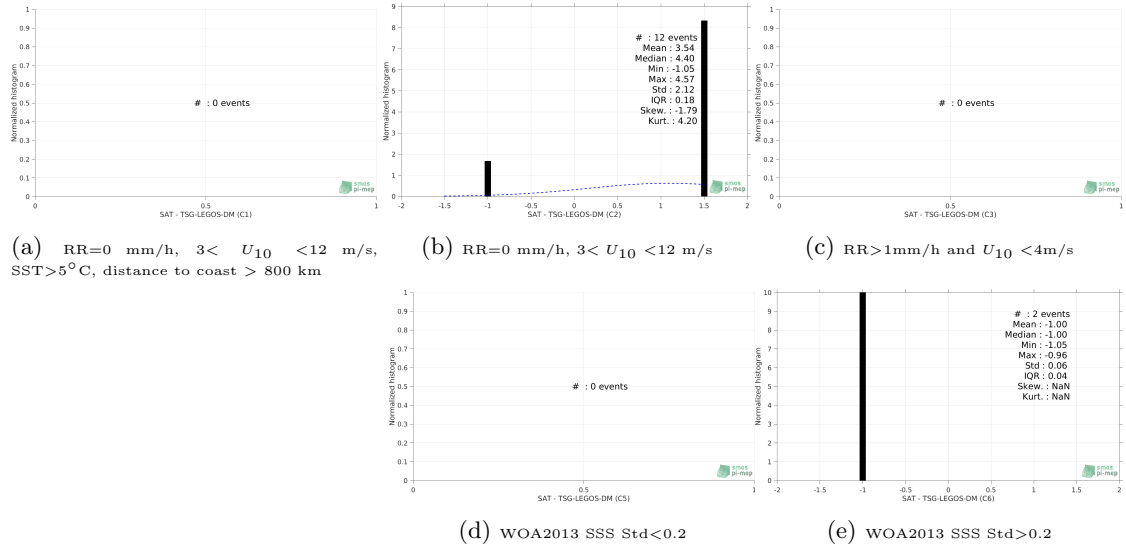
Figure 13: Normalized histogram of \Delta SSS (SMOS-L3-CATDS-CPDC-V321-L2Q - TSG-LEGOS-DM) for 5 different subdatasets corresponding to: RR=0 mm/h, 3 < U_{10} < 12 m/s, SST>5°C, distance to coast > 800 km (a), RR=0 mm/h, 3 < U_{10} < 12 m/s (b), RR>1mm/h and U_{10} < 4 m/s (c), WOA2013 SSS Std<0.2 (d), WOA2013 SSS Std>0.2 (e).
