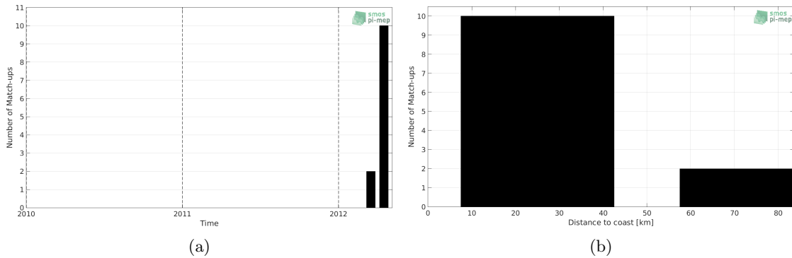
Figure 1: Number of match-ups between TSG-LEGOS-DM and SMOS-L3-CATDS-CPDC-V321-L2Q SSS as a function of time (a) and as function of the distance to coast (b) over the Mediterranean Sea Pi-MEP region and for the full satellite product period.
