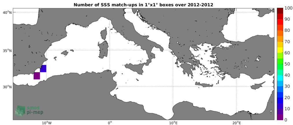
Figure 4: Number of SSS match-ups between TSG-LEGOS-DM SSS and the SMOS-L3-CATDS-CPDC-V321-L2Q SSS product for the Mediterranean Sea Pi-MEP region over 1^\circ \times 1^\circ boxes and for the full satellite product period.
