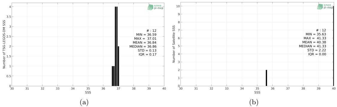
Figure 2: Histograms of SSS from TSG-LEGOS-DM (a) and SMOS-L3-CATDS-CPDC-V321-L2Q (b) considering all match-up pairs per bins of 0.1 over the Mediterranean Sea Pi-MEP region and for the full satellite product period.
