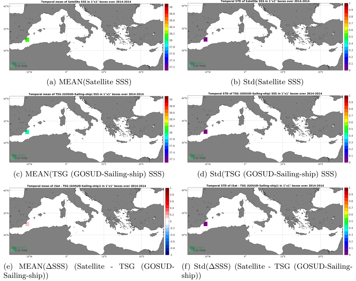
Figure 6: Temporal mean (left) and Std (right) of SSS from SMOS SSS L2Q v321 - 0.25 Deg (CATDS-CPDC) (top), TSG (GOSUD-Sailing-ship) (middle), and of \Delta\text{SSS} (Satellite - TSG (GOSUD-Sailing-ship)). Only match-up pairs are used to generate these maps.
