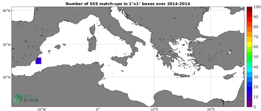
Figure 4: Number of SSS match-ups between TSG (GOSUD-Sailing-ship) SSS and the SMOS SSS L2Q v321 - 0.25 Deg (CATDS-CPDC) SSS product for the Mediterranean Sea Pi-MEP region over 1^\circ \times 1^\circ boxes and for the full satellite product period.
