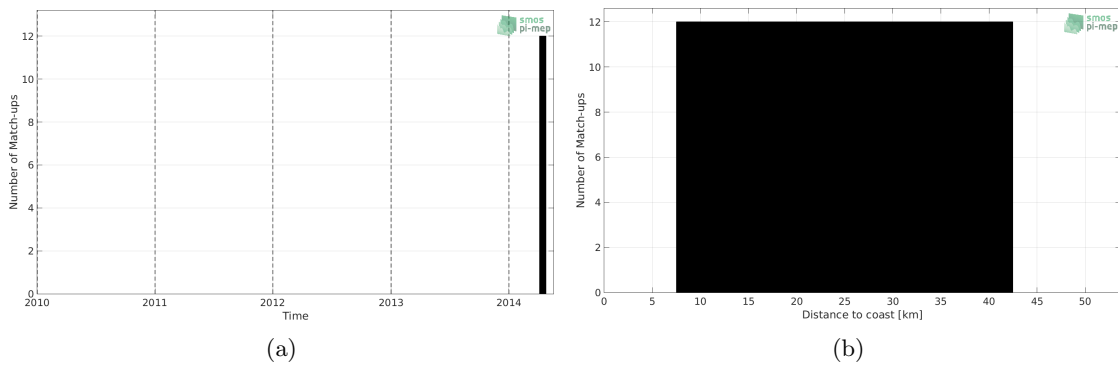
Figure 1: Number of match-ups between TSG (GOSUD-Sailing-ship) and SMOS SSS L2Q v321 - 0.25 Deg (CATDS-CPDC) SSS as a function of time (a) and as function of the distance to coast (b) over the Mediterranean Sea Pi-MEP region and for the full satellite product period.
