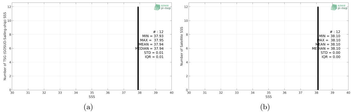
Figure 2: Histograms of SSS from TSG (GOSUD-Sailing-ship) (a) and SMOS SSS L2Q v321 - 0.25 Deg (CATDS-CPDC) (b) considering all match-up pairs per bins of 0.1 over the Mediterranean Sea Pi-MEP region and for the full satellite product period.
