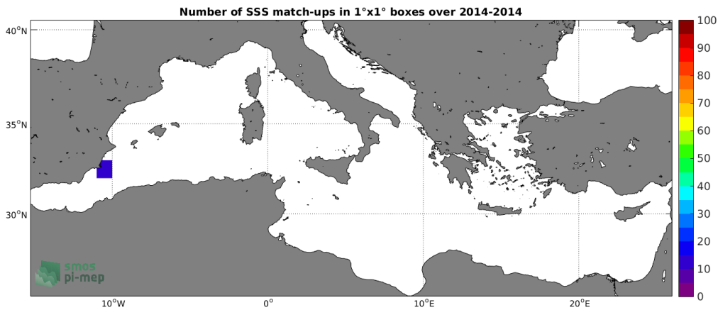
Figure 4: Number of SSS match-ups between TSG (GOSUD-Sailing-ship) SSS and the SMOS SSS L2Q v321 - 0.25 Deg (CATDS-CPDC) SSS product for the Mediterranean Sea Pi-MEP region over 1°x1° boxes and for the full satellite product period.
