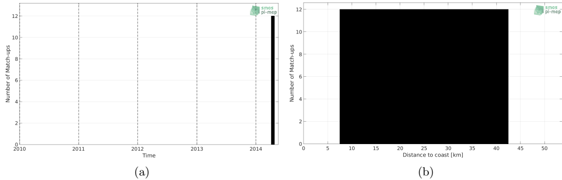
Figure 1: Number of match-ups between TSG (GOSUD-Sailing-ship) and SMOS SSS L2Q v321 - 0.25 Deg (CATDS-CPDC) SSS as a function of time (a) and as function of the distance to coast (b) over the Mediterranean Sea Pi-MEP region and for the full satellite product period.
