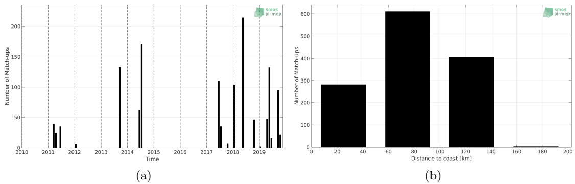
Figure 1: Number of match-ups between TSG (GOSUD-Research-vessel) and SMOS SSS L2Q v321 - 0.25 Deg (CATDS-CPDC) SSS as a function of time (a) and as function of the distance to coast (b) over the Mediterranean Sea Pi-MEP region and for the full satellite product period.
