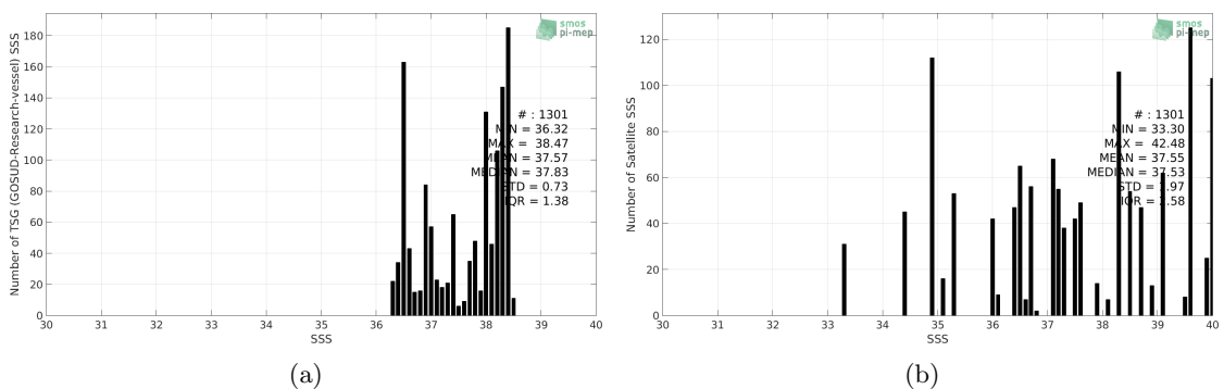
Figure 2: Histograms of SSS from TSG (GOSUD-Research-vessel) (a) and SMOS SSS L2Q v321 - 0.25 Deg (CATDS-CPDC) (b) considering all match-up pairs per bins of 0.1 over the Mediterranean Sea Pi-MEP region and for the full satellite product period.
