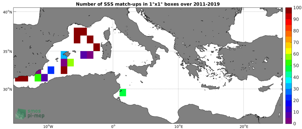
Figure 4: Number of SSS match-ups between TSG (GOSUD-Research-vessel) SSS and the SMOS SSS L2Q v321 - 0.25 Deg (CATDS-CPDC) SSS product for the Mediterranean Sea Pi-MEP region over 1^\circ \times 1^\circ boxes and for the full satellite product period.
