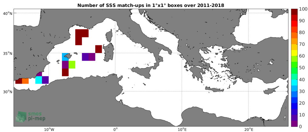
Figure 4: Number of SSS match-ups between TSG (GOSUD-Research-vessel) SSS and the SMOS SSS L2Q v321 - 0.25 Deg (CATDS-CPDC) SSS product for the Mediterranean Sea Pi-MEP region over 1°x1° boxes and for the full satellite product period.
