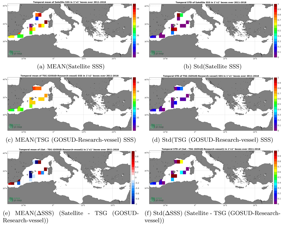
Figure 6: Temporal mean (left) and Std (right) of SSS from SMOS SSS L2Q v321 - 0.25 Deg (CATDS-CPDC) (top), TSG (GOSUD-Research-vessel) (middle), and of \Delta SSS (Satellite - TSG (GOSUD-Research-vessel)). Only match-up pairs are used to generate these maps.
