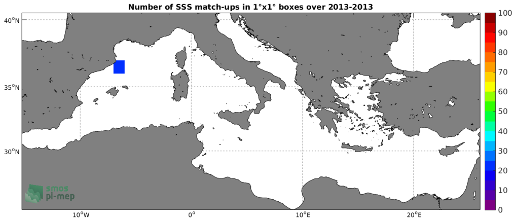
Figure 3: Number of SSS match-ups between Surface drifters SSS and the SMOS SSS L2Q v321 - 0.25 Deg (CATDS-CPDC) SSS product for the Mediterranean Sea Pi-MEP region over 1^\circ \times 1^\circ boxes and for the full satellite product period.
