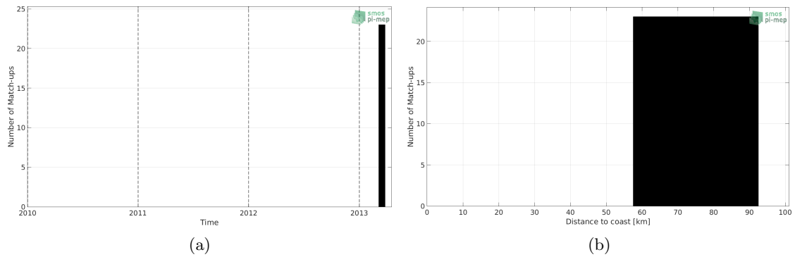
Figure 1: Number of match-ups between Surface drifters and SMOS SSS L2Q v321 - 0.25 Deg (CATDS-CPDC) SSS as a function of time (a) and as function of the distance to coast (b) over the Mediterranean Sea Pi-MEP region and for the full satellite product period.
