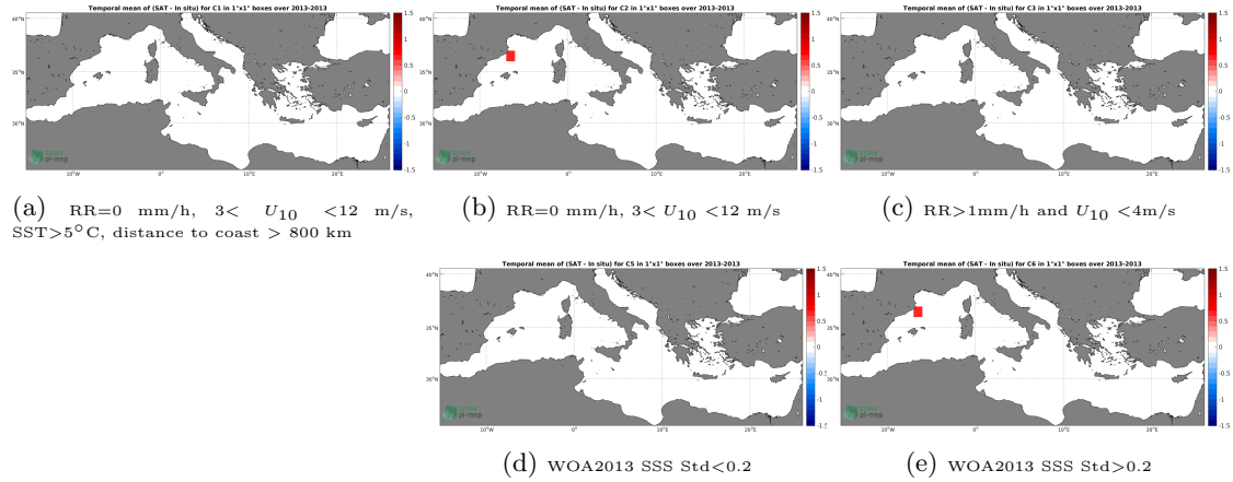
Figure 11: Temporal mean gridded over spatial boxes of size 1^{\circ}\times 1^{\circ} of \Delta\text{SSS} (SMOS SSS L2Q v321 - 0.25 Deg (CATDS-CPDC) - Surface drifters) for 5 different subdatasets corresponding to:RR=0 mm/h, 3 < U_{10} < 12 m/s, SST >5^{\circ}\text{C} , distance to coast > 800 km (a), RR=0 mm/h, 3 < U_{10} < 12 m/s (b), RR >1 mm/h and U_{10} < 4 m/s (c), WOA2013 SSS Std <0.2 (d), WOA2013 SSS Std >0.2 (e).
