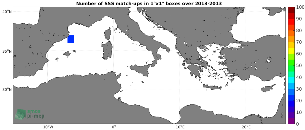
Figure 3: Number of SSS match-ups between Surface drifters SSS and the SMOS SSS L2Q v321 - 0.25 Deg (CATDS-CPDC) SSS product for the Mediterranean Sea Pi-MEP region over 1°x1° boxes and for the full satellite product period.
