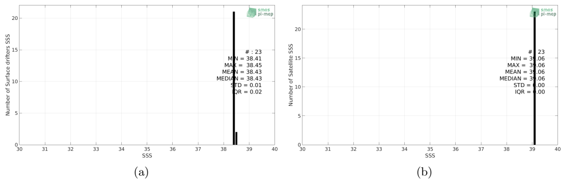
Figure 2: Histograms of SSS from Surface drifters (a) and SMOS SSS L2Q v321 - 0.25 Deg (CATDS-CPDC) (b) considering all match-up pairs per bins of 0.1 over the Mediterranean Sea Pi-MEP region and for the full satellite product period.
