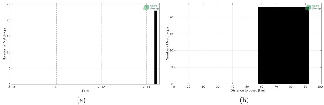
Figure 1: Number of match-ups between Surface drifters and SMOS SSS L2Q v321 - 0.25 Deg (CATDS-CPDC) SSS as a function of time (a) and as function of the distance to coast (b) over the Mediterranean Sea Pi-MEP region and for the full satellite product period.
