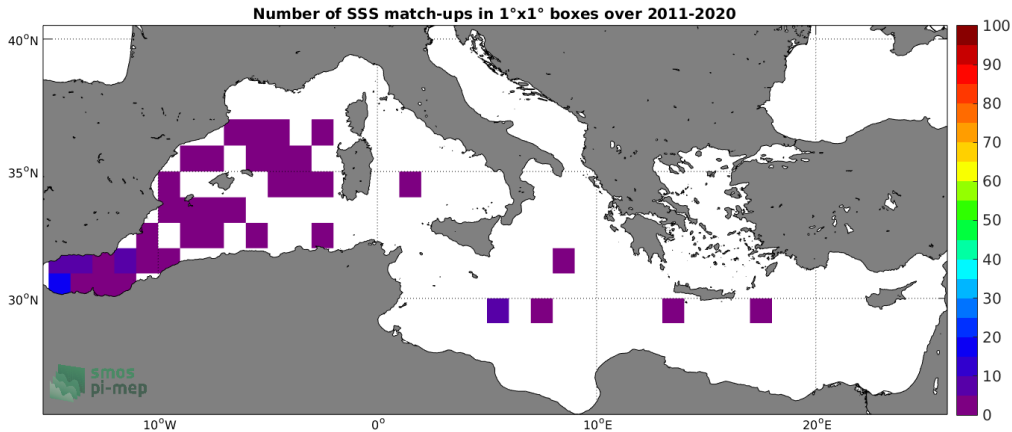
Figure 4: Number of SSS match-ups between Argo SSS and the SMOS SSS L2Q v321 - 0.25 Deg (CATDS-CPDC) SSS product for the Mediterranean Sea Pi-MEP region over 1^\circ \times 1^\circ boxes and for the full satellite product period.
