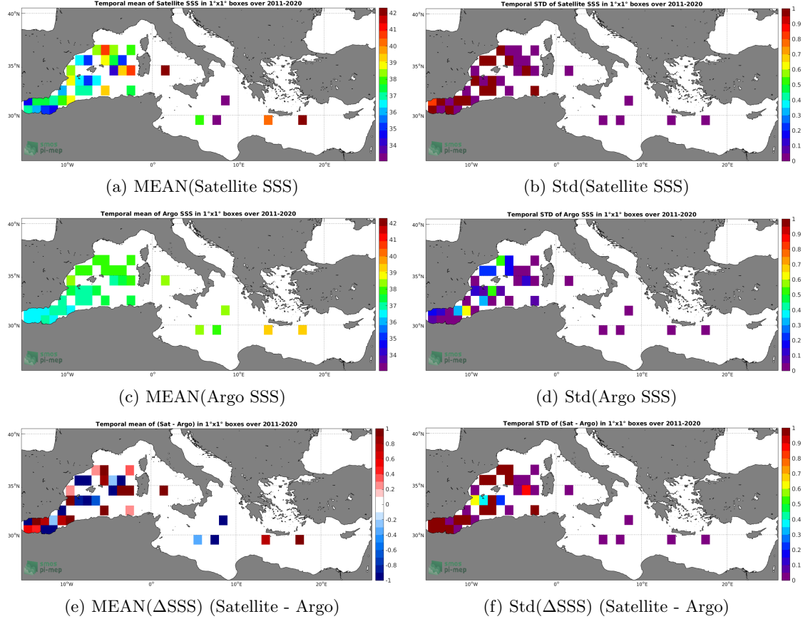
Figure 6: Temporal mean (left) and Std (right) of SSS from SMOS SSS L2Q v321 - 0.25 Deg (CATDS-CPDC) (top), Argo (middle), and of \Delta\text{SSS} (Satellite - Argo). Only match-up pairs are used to generate these maps.
