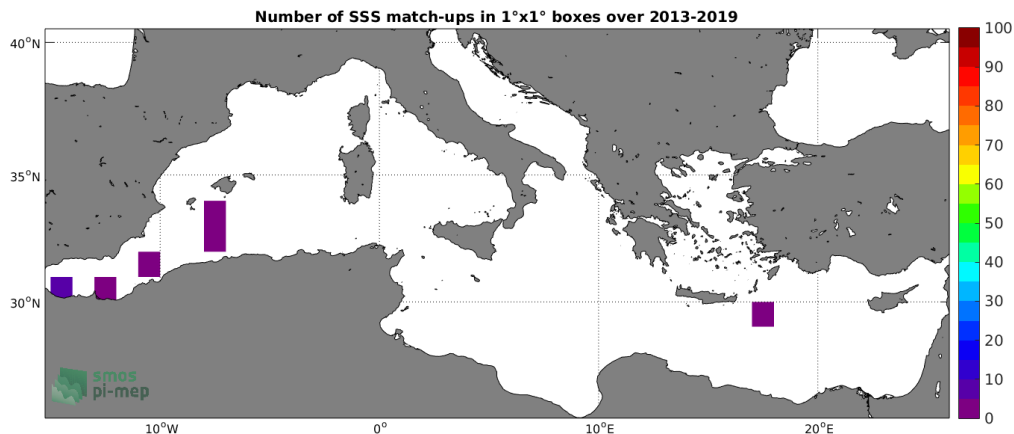
Figure 4: Number of SSS match-ups between Argo SSS and the SMOS-L3-CATDS-CPDC-V321-L2Q SSS product for the Mediterranean Sea Pi-MEP region over 1°x1° boxes and for the full satellite product period.
