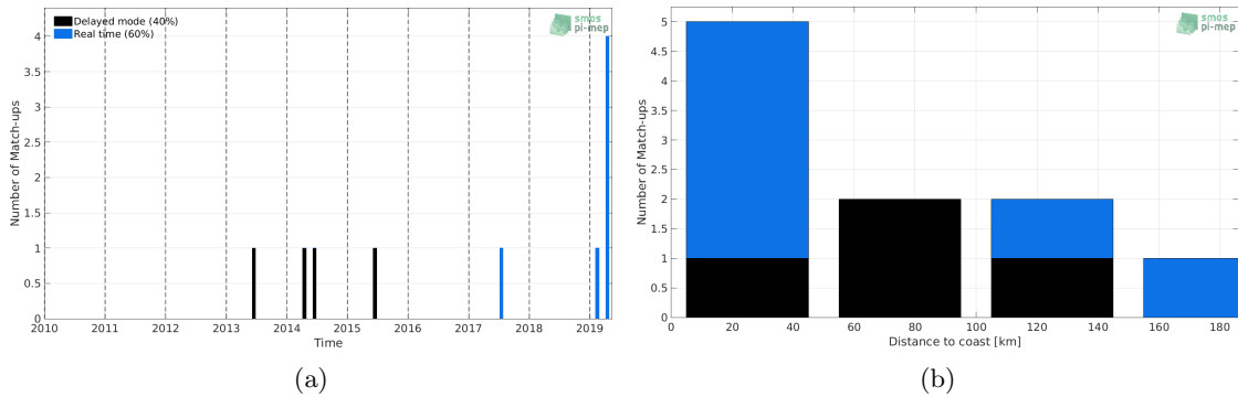
Figure 1: Number of match-ups between Argo and SMOS-L3-CATDS-CPDC-V321-L2Q SSS as a function of time (a) and as function of the distance to coast (b) over the Mediterranean Sea Pi-MEP region and for the full satellite product period.
