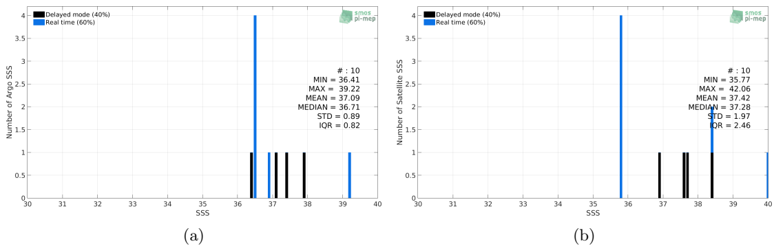
Figure 2: Histograms of SSS from Argo (a) and SMOS-L3-CATDS-CPDC-V321-L2Q (b) considering all match-up pairs per bins of 0.1 over the Mediterranean Sea Pi-MEP region and for the full satellite product period.
