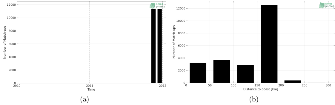
Figure 1: Number of match-ups between TSG (SAMOS) and SMOS SSS L3 v317 - Monthly - 25 km (CATDS-CPDC) SSS as a function of time (a) and as function of the distance to coast (b) over the Mediterranean Sea Pi-MEP region and for the full satellite product period.
