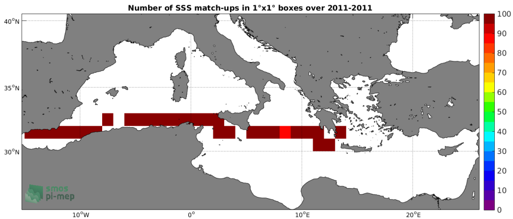
Figure 4: Number of SSS match-ups between TSG (SAMOS) SSS and the SMOS SSS L3 v317 - Monthly - 25 km (CATDS-CPDC) SSS product for the Mediterranean Sea Pi-MEP region over 1^\circ \times 1^\circ boxes and for the full satellite product period.
