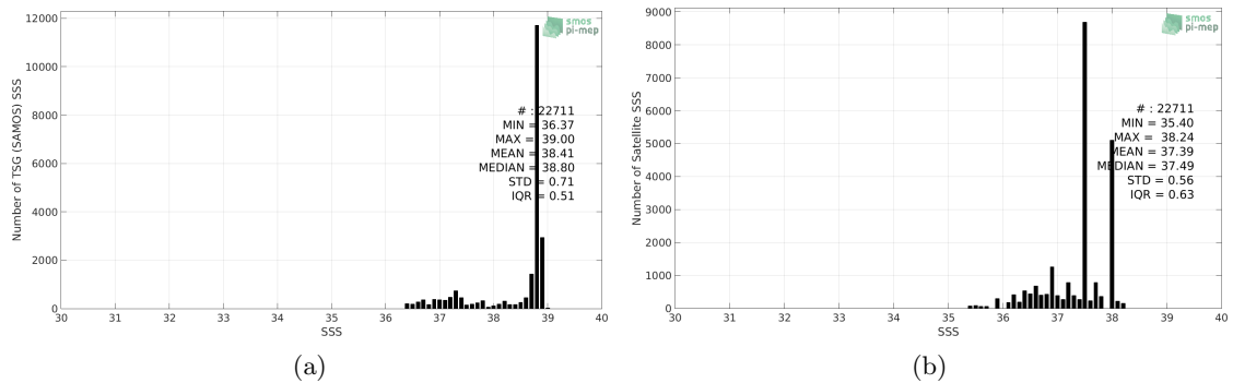
Figure 2: Histograms of SSS from TSG (SAMOS) (a) and SMOS SSS L3 v317 - Monthly - 25 km (CATDS-CPDC) (b) considering all match-up pairs per bins of 0.1 over the Mediterranean Sea Pi-MEP region and for the full satellite product period.
