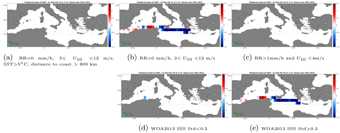
Figure 12: Temporal mean gridded over spatial boxes of size 1^{\circ}\times 1^{\circ} of \Delta\text{SSS} (SMOS SSS L3 v317 - Monthly - 25 km (CATDS-CPDC) - TSG (SAMOS)) for 5 different subdatasets corresponding to:RR=0 mm/h, 3 < U_{10} < 12 m/s, SST >5^{\circ}\text{C} , distance to coast > 800 km (a), RR=0 mm/h, 3 < U_{10} < 12 m/s (b), RR >1 mm/h and U_{10} < 4 m/s (c), WOA2013 SSS Std <0.2 (d), WOA2013 SSS Std >0.2 (e).
