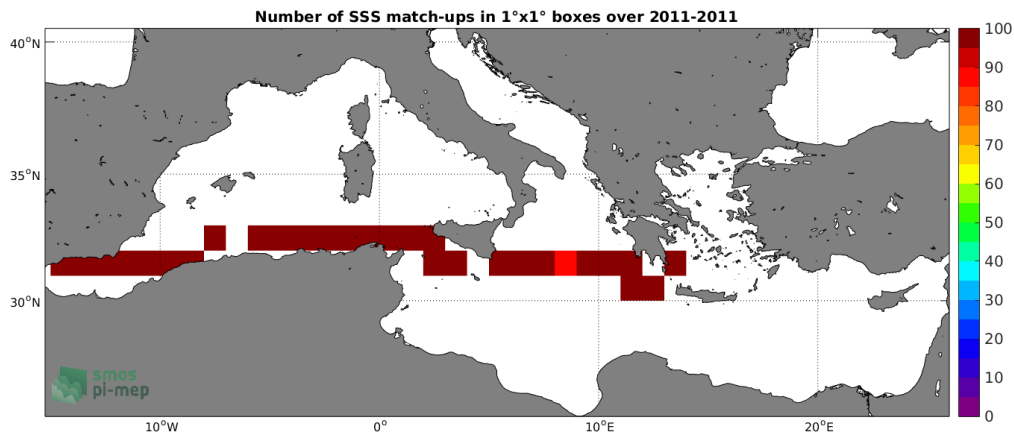
Figure 4: Number of SSS match-ups between TSG-SAMOS SSS and the SMOS L3 v317 - Monthly - 25 km (CATDS-CPDC) SSS product for the Mediterranean Sea Pi-MEP region over 1^\circ \times 1^\circ boxes and for the full satellite product period.
