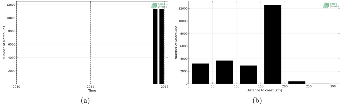
Figure 1: Number of match-ups between TSG-SAMOS and SMOS L3 v317 - Monthly - 25 km (CATDS-CPDC) SSS as a function of time (a) and as function of the distance to coast (b) over the Mediterranean Sea Pi-MEP region and for the full satellite product period.
