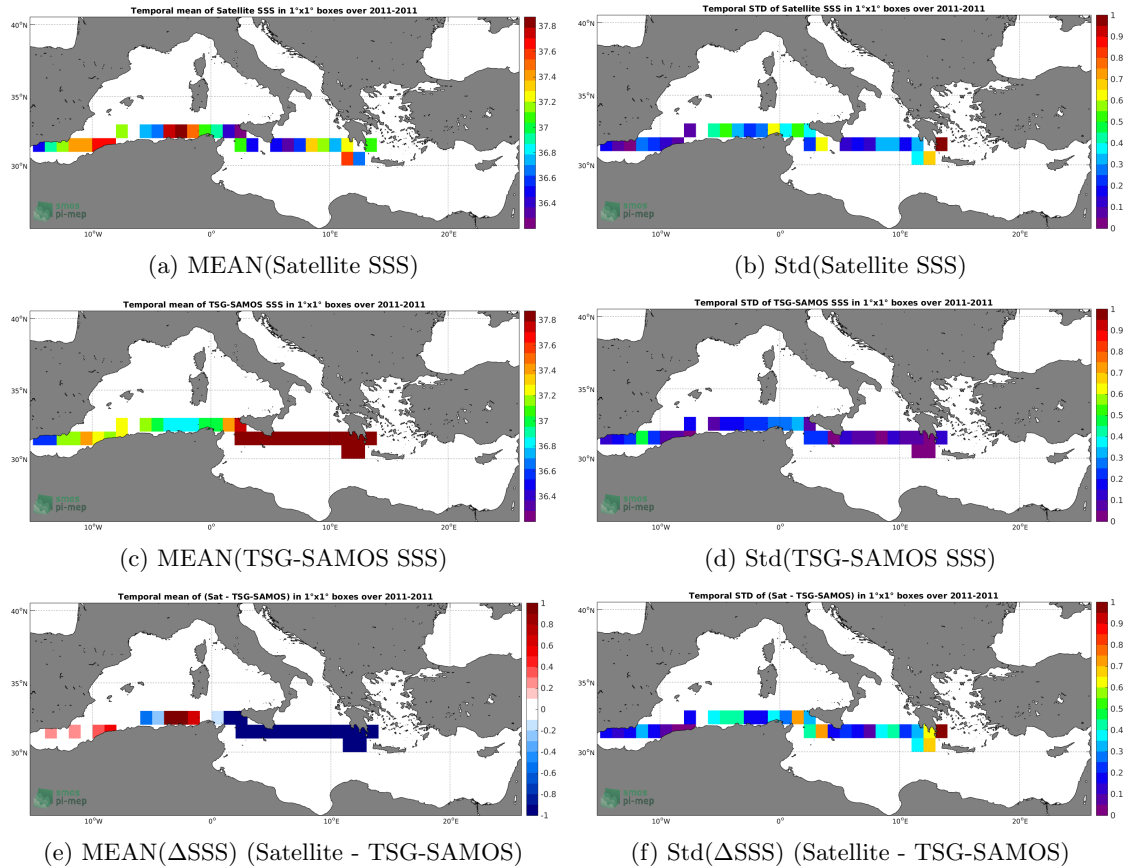
Figure 6: Temporal mean (left) and Std (right) of SSS from SMOS L3 v317 - Monthly - 25 km (CATDS-CPDC) (top), TSG-SAMOS (middle), and of \Delta SSS (Satellite - TSG-SAMOS). Only match-up pairs are used to generate these maps.
