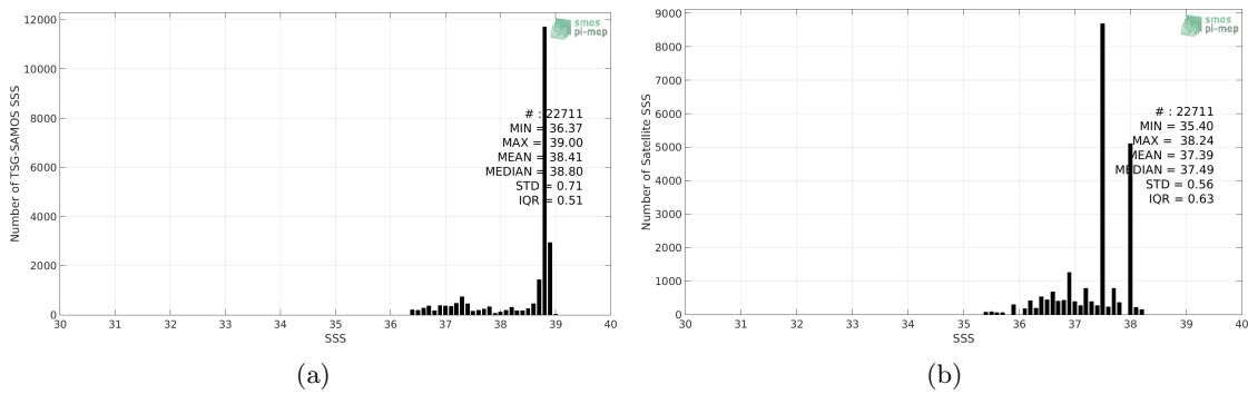
Figure 2: Histograms of SSS from TSG-SAMOS (a) and SMOS L3 v317 - Monthly - 25 km (CATDS-CPDC) (b) considering all match-up pairs per bins of 0.1 over the Mediterranean Sea Pi-MEP region and for the full satellite product period.
