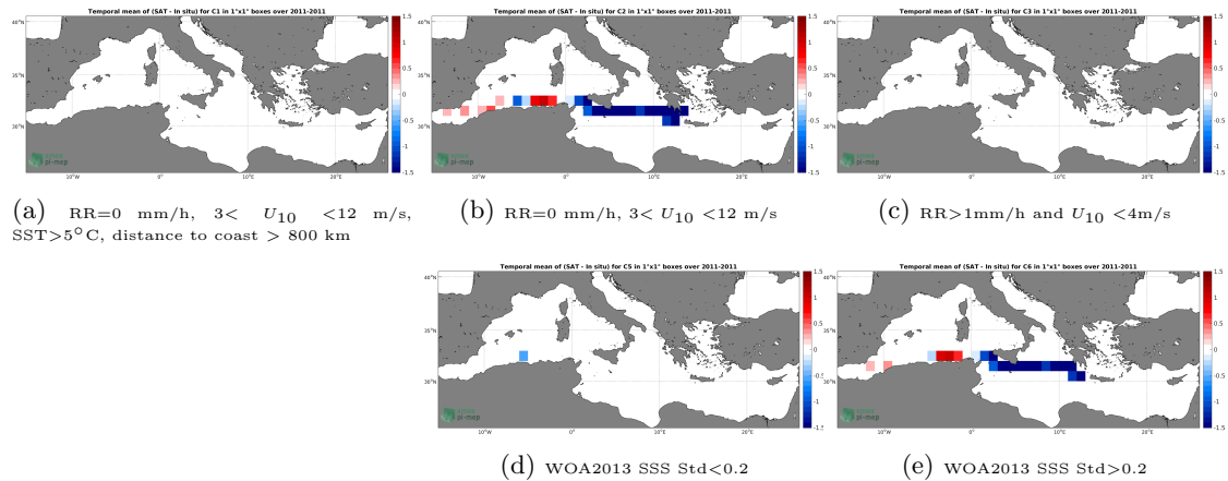
Figure 12: Temporal mean gridded over spatial boxes of size 1^{\circ}\times 1^{\circ} of \Delta\text{SSS} (SMOS L3 v317 - Monthly - 25 km (CATDS-CPDC) - TSG-SAMOS) for 5 different subdatasets corresponding to:RR=0 mm/h, 3 < U_{10} < 12 m/s, SST > 5^{\circ}\text{C} , distance to coast > 800 km (a), RR=0 mm/h, 3 < U_{10} < 12 m/s (b), RR > 1 mm/h and U_{10} < 4 m/s (c), WOA2013 SSS Std < 0.2 (d), WOA2013 SSS Std > 0.2 (e).
