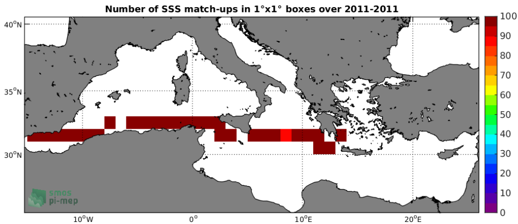
Figure 4: Number of SSS match-ups between TSG-SAMOS SSS and the SMOS-L3-CATDS-CPDC-V317-MONTHLY-25KM SSS product for the Mediterranean Sea Pi-MEP region over 1^\circ \times 1^\circ boxes and for the full satellite product period.
