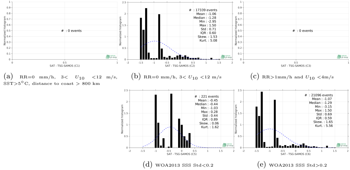
Figure 13: Normalized histogram of \Delta\text{SSS} (SMOS-L3-CATDS-CPDC-V317-MONTHLY-25KM - TSG-SAMOS) for 5 different subdatasets corresponding to: RR=0 mm/h, 3 < U_{10} < 12 m/s, SST > 5^\circ\text{C} , distance to coast > 800 km (a), RR=0 mm/h, 3 < U_{10} < 12 m/s (b), RR > 1 mm/h and U_{10} < 4 m/s (c), WOA2013 SSS Std < 0.2 (d), WOA2013 SSS Std > 0.2 (e).
