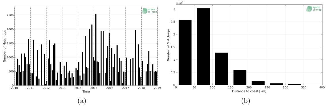
Figure 1: Number of match-ups between TSG-LEGOS-DM and SMOS L3 v317 - Monthly - 25 km (CATDS-CPDC) SSS as a function of time (a) and as function of the distance to coast (b) over the Mediterranean Sea Pi-MEP region and for the full satellite product period.
