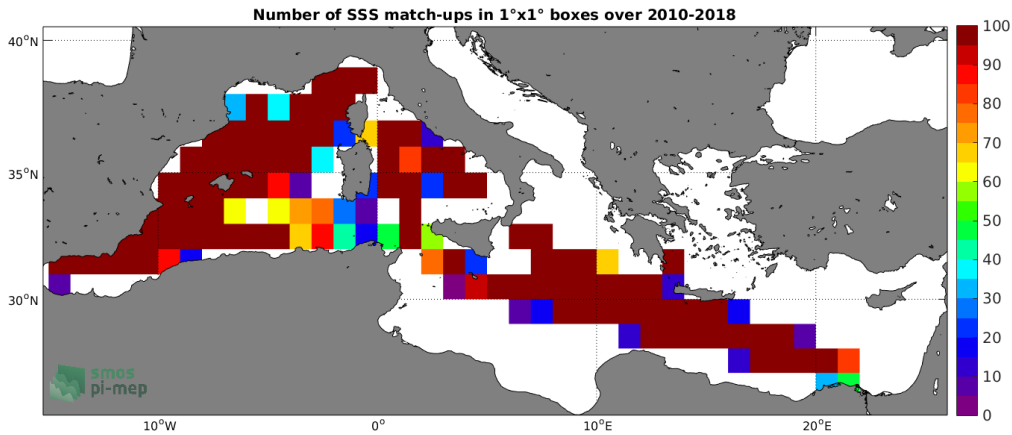
Figure 4: Number of SSS match-ups between TSG-LEGOS-DM SSS and the SMOS L3 v317 - Monthly - 25 km (CATDS-CPDC) SSS product for the Mediterranean Sea Pi-MEP region over 1°x1° boxes and for the full satellite product period.
