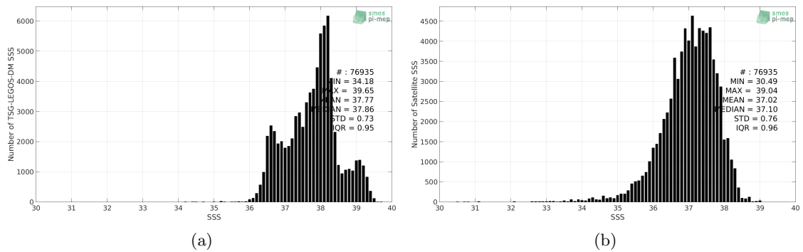
Figure 2: Histograms of SSS from TSG-LEGOS-DM (a) and SMOS L3 v317 - Monthly - 25 km (CATDS-CPDC) (b) considering all match-up pairs per bins of 0.1 over the Mediterranean Sea Pi-MEP region and for the full satellite product period.
