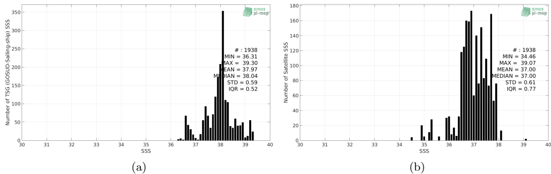
Figure 2: Histograms of SSS from TSG (GOSUD-Sailing-ship) (a) and SMOS SSS L3 v317 - Monthly - 25 km (CATDS-CPDC) (b) considering all match-up pairs per bins of 0.1 over the Mediterranean Sea Pi-MEP region and for the full satellite product period.
