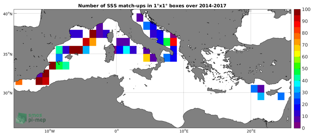
Figure 4: Number of SSS match-ups between TSG (GOSUD-Sailing-ship) SSS and the SMOS SSS L3 v317 - Monthly - 25 km (CATDS-CPDC) SSS product for the Mediterranean Sea Pi-MEP region over 1^\circ \times 1^\circ boxes and for the full satellite product period.
