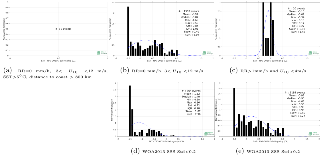
Figure 13: Normalized histogram of \Delta SSS (SMOS L3 v317 - Monthly - 25 km (CATDS-CPDC) - TSG-GOSUD-Sailing-ship) for 5 different subdatasets corresponding to: RR=0 mm/h, 3 < U_{10} < 12 m/s, SST > 5°C, distance to coast > 800 km (a), RR=0 mm/h, 3 < U_{10} < 12 m/s (b), RR > 1mm/h and U_{10} < 4 m/s (c), WOA2013 SSS Std < 0.2 (d), WOA2013 SSS Std > 0.2 (e).
