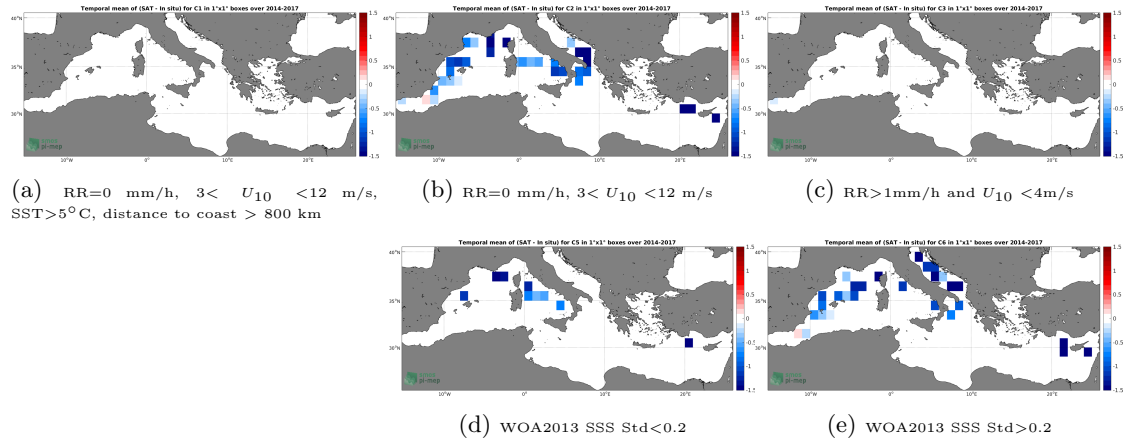
Figure 12: Temporal mean gridded over spatial boxes of size 1^{\circ}\times 1^{\circ} of \Delta SSS (SMOS L3 v317 - Monthly - 25 km (CATDS-CPDC) - TSG-GOSUD-Sailing-ship) for 5 different subdatasets corresponding to:RR=0 mm/h, 3 < U_{10} < 12 m/s, SST >5^{\circ}\text{C} , distance to coast > 800 km (a), RR=0 mm/h, 3 < U_{10} < 12 m/s (b), RR >1 mm/h and U_{10} < 4 m/s (c), WOA2013 SSS Std <0.2 (d), WOA2013 SSS Std >0.2 (e).
