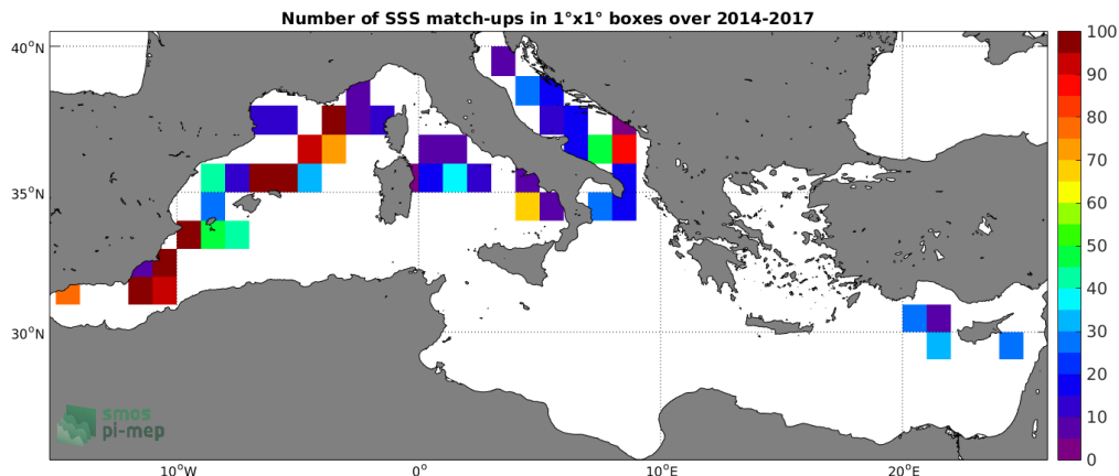
Figure 4: Number of SSS match-ups between TSG-GOSUD-Sailing-ship SSS and the SMOS L3 v317 - Monthly - 25 km (CATDS-CPDC) SSS product for the Mediterranean Sea Pi-MEP region over 1°x1° boxes and for the full satellite product period.
