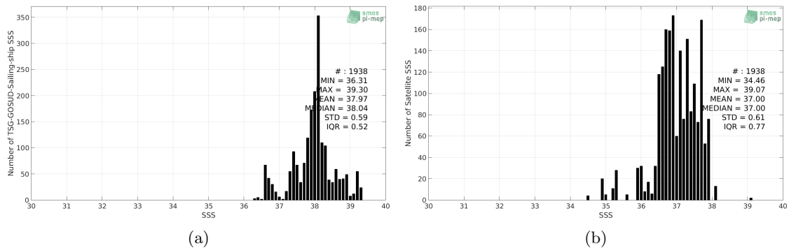
Figure 2: Histograms of SSS from TSG-GOSUD-Sailing-ship (a) and SMOS L3 v317 - Monthly - 25 km (CATDS-CPDC) (b) considering all match-up pairs per bins of 0.1 over the Mediterranean Sea Pi-MEP region and for the full satellite product period.
