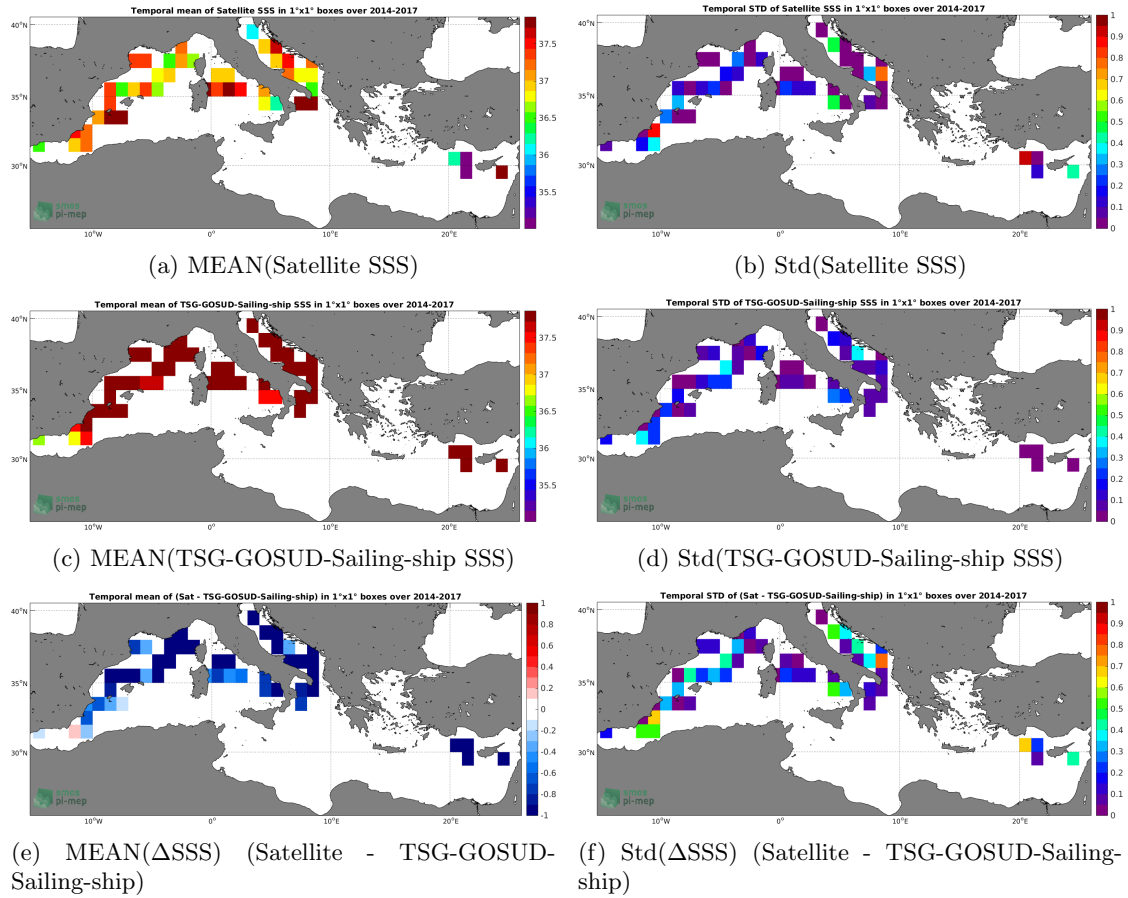
Figure 6: Temporal mean (left) and Std (right) of SSS from SMOS L3 v317 - Monthly - 25 km (CATDS-CPDC) (top), TSG-GOSUD-Sailing-ship (middle), and of \Delta SSS (Satellite - TSG-GOSUD-Sailing-ship). Only match-up pairs are used to generate these maps.
