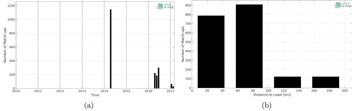
Figure 1: Number of match-ups between TSG-GOSUD-Sailing-ship and SMOS-L3-CATDS-CPDC-V317-MONTHLY-25KM SSS as a function of time (a) and as function of the distance to coast (b) over the Mediterranean Sea Pi-MEP region and for the full satellite product period.
