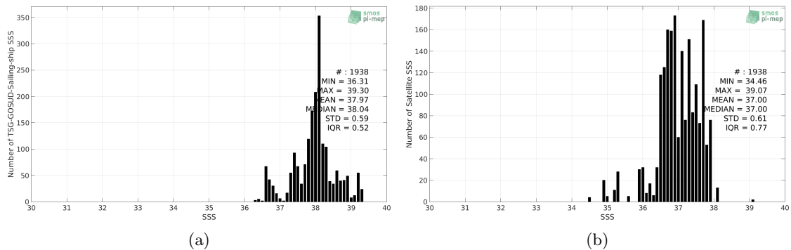
Figure 2: Histograms of SSS from TSG-GOSUD-Sailing-ship (a) and SMOS-L3-CATDS-CPDC-V317-MONTHLY-25KM (b) considering all match-up pairs per bins of 0.1 over the Mediterranean Sea Pi-MEP region and for the full satellite product period.
