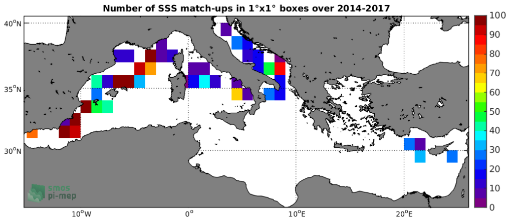
Figure 4: Number of SSS match-ups between TSG-GOSUD-Sailing-ship SSS and the SMOS-L3-CATDS-CPDC-V317-MONTHLY-25KM SSS product for the Mediterranean Sea Pi-MEP region over 1^\circ \times 1^\circ boxes and for the full satellite product period.
