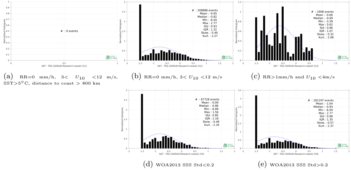
Figure 13: Normalized histogram of \Delta\text{SSS} (SMOS SSS L3 v317 - Monthly - 25 km (CATDS-CPDC) - TSG (GOSUD-Research-vessel)) for 5 different subdatasets corresponding to: RR=0 mm/h, 3 < U_{10} < 12 m/s, SST > 5^\circ\text{C} , distance to coast > 800 km (a), RR=0 mm/h, 3 < U_{10} < 12 m/s (b), RR > 1\text{mm/h} and U_{10} < 4\text{m/s} (c), WOA2013 SSS Std < 0.2 (d), WOA2013 SSS Std > 0.2 (e).
