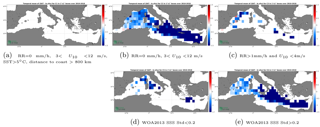
Figure 12: Temporal mean gridded over spatial boxes of size 1^\circ \times 1^\circ of \Delta SSS (SMOS-L3-CATDS-CPDC-V317-MONTHLY-25KM - TSG-GOSUD-Research-vessel) for 5 different subdatasets corresponding to: RR=0 mm/h, 3 < U_{10} < 12 m/s, SST >5^\circ\text{C} , distance to coast > 800 km (a), RR=0 mm/h, 3 < U_{10} < 12 m/s (b), RR >1 mm/h and U_{10} < 4 m/s (c), WOA2013 SSS Std <0.2 (d), WOA2013 SSS Std >0.2 (e).
