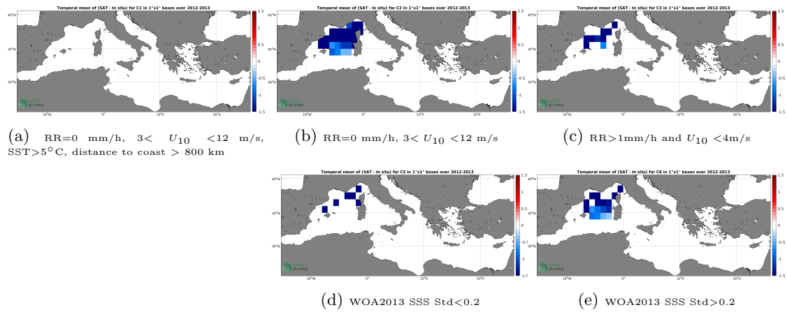
Figure 11: Temporal mean gridded over spatial boxes of size 1^\circ \times 1^\circ of \Delta SSS (SMOS SSS L3 v317 - Monthly - 25 km (CATDS-CPDC) - Surface drifters) for 5 different subdatasets corresponding to:RR=0 mm/h, 3 < U_{10} < 12 m/s, SST >5^\circ C, distance to coast > 800 km (a), RR=0 mm/h, 3 < U_{10} < 12 m/s (b), RR >1 mm/h and U_{10} < 4 m/s (c), WOA2013 SSS Std <0.2 (d), WOA2013 SSS Std >0.2 (e).
