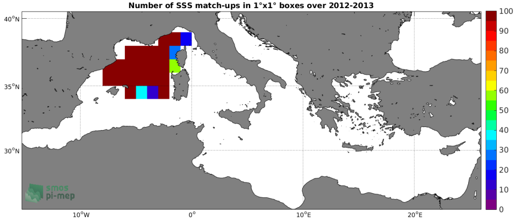
Figure 3: Number of SSS match-ups between Surface drifters SSS and the SMOS L3 v317 - Monthly - 25 km (CATDS-CPDC) SSS product for the Mediterranean Sea Pi-MEP region over 1°x1° boxes and for the full satellite product period.
