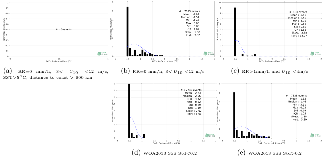
Figure 12: Normalized histogram of \Delta\text{SSS} (SMOS L3 v317 - Monthly - 25 km (CATDS-CPDC) - Surface drifters) for 5 different subdatasets corresponding to: RR=0 mm/h, 3 < U_{10} < 12 m/s, SST > 5^{\circ}\text{C} , distance to coast > 800 km (a), RR=0 mm/h, 3 < U_{10} < 12 m/s (b), RR > 1\text{mm/h} and U_{10} < 4\text{m/s} (c), WOA2013 SSS Std < 0.2 (d), WOA2013 SSS Std > 0.2 (e).
