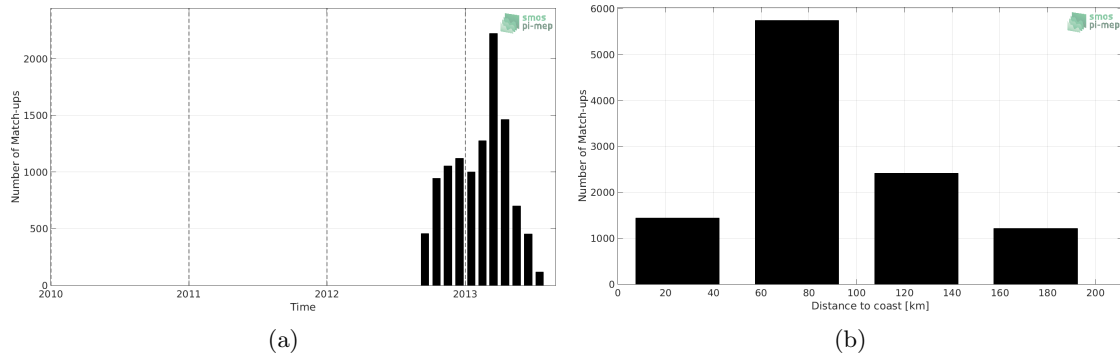
Figure 1: Number of match-ups between Surface drifters and SMOS L3 v317 - Monthly - 25 km (CATDS-CPDC) SSS as a function of time (a) and as function of the distance to coast (b) over the Mediterranean Sea Pi-MEP region and for the full satellite product period.
