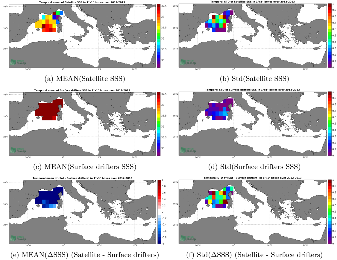
Figure 5: Temporal mean (left) and Std (right) of SSS from SMOS L3 v317 - Monthly - 25 km (CATDS-CPDC) (top), Surface drifters (middle), and of \Delta SSS (Satellite - Surface drifters). Only match-up pairs are used to generate these maps.
