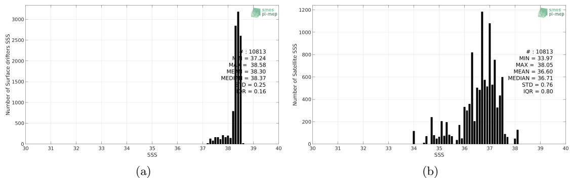
Figure 2: Histograms of SSS from Surface drifters (a) and SMOS L3 v317 - Monthly - 25 km (CATDS-CPDC) (b) considering all match-up pairs per bins of 0.1 over the Mediterranean Sea Pi-MEP region and for the full satellite product period.
