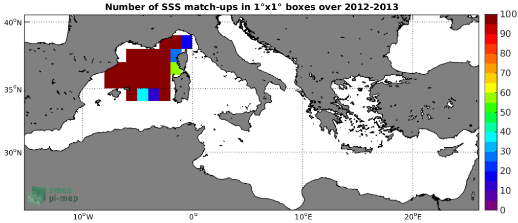
Figure 3: Number of SSS match-ups between Surface drifters SSS and the SMOS-L3-CATDS-CPDC-V317-MONTHLY-25KM SSS product for the Mediterranean Sea Pi-MEP region over 1°x1° boxes and for the full satellite product period.
