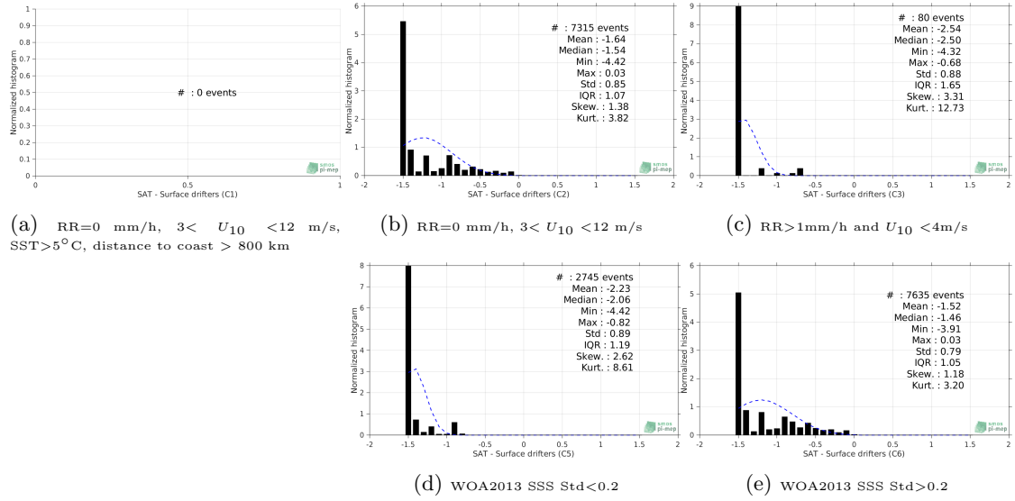
Figure 12: Normalized histogram of \Delta\text{SSS} (SMOS-L3-CATDS-CPDC-V317-MONTHLY-25KM - Surface drifters) for 5 different subdatasets corresponding to: RR=0 mm/h, 3 < U_{10} < 12 m/s, SST > 5^{\circ}\text{C} , distance to coast > 800 km (a), RR=0 mm/h, 3 < U_{10} < 12 m/s (b), RR > 1\text{mm/h} and U_{10} < 4\text{m/s} (c), WOA2013 SSS Std < 0.2 (d), WOA2013 SSS Std > 0.2 (e).
