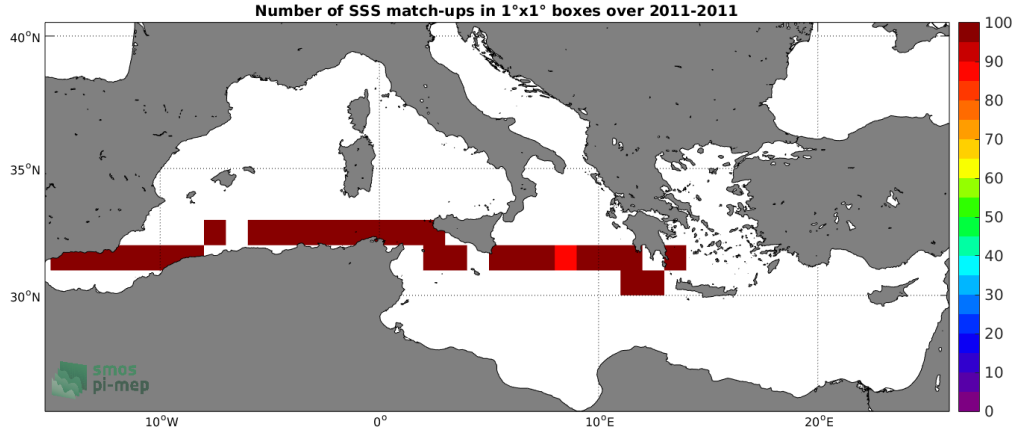
Figure 4: Number of SSS match-ups between TSG (SAMOS) SSS and the SMOS SSS L3 v317 - 10 Days - 25 km (CATDS-CPDC) SSS product for the Mediterranean Sea Pi-MEP region over 1^\circ \times 1^\circ boxes and for the full satellite product period.
