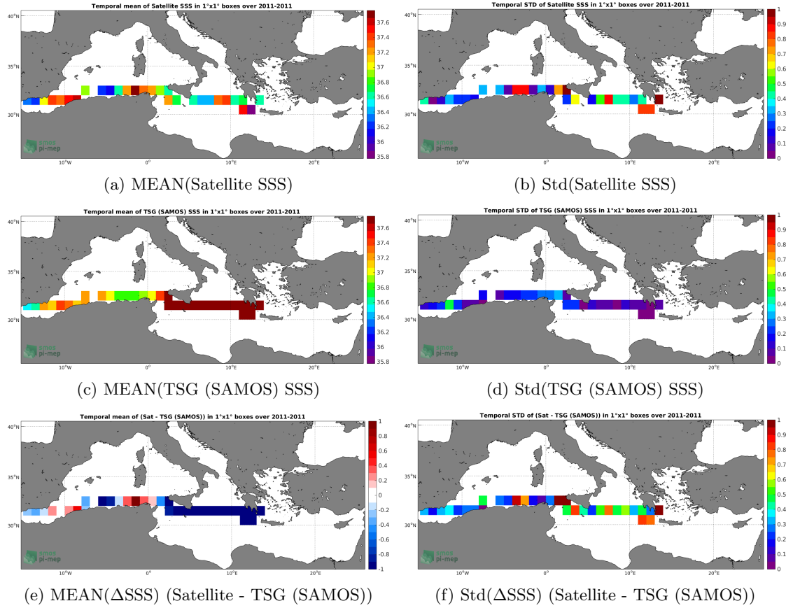
Figure 6: Temporal mean (left) and Std (right) of SSS from SMOS SSS L3 v317 - 10 Days - 25 km (CATDS-CPDC) (top), TSG (SAMOS) (middle), and of \Delta SSS (Satellite - TSG (SAMOS)). Only match-up pairs are used to generate these maps.
