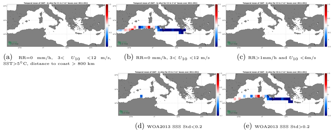
Figure 12: Temporal mean gridded over spatial boxes of size 1^{\circ}\times 1^{\circ} of \Delta\text{SSS} (SMOS SSS L3 v317 - 10 Days - 25 km (CATDS-CPDC) - TSG (SAMOS)) for 5 different subdatasets corresponding to: RR=0 mm/h, 3 < U_{10} < 12 m/s, SST > 5^{\circ}\text{C} , distance to coast > 800 km (a), RR=0 mm/h, 3 < U_{10} < 12 m/s (b), RR > 1 mm/h and U_{10} < 4 m/s (c), WOA2013 SSS Std < 0.2 (d), WOA2013 SSS Std > 0.2 (e).
