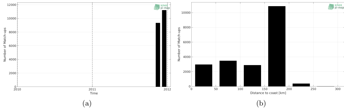
Figure 1: Number of match-ups between TSG (SAMOS) and SMOS SSS L3 v317 - 10 Days - 25 km (CATDS-CPDC) SSS as a function of time (a) and as function of the distance to coast (b) over the Mediterranean Sea Pi-MEP region and for the full satellite product period.
