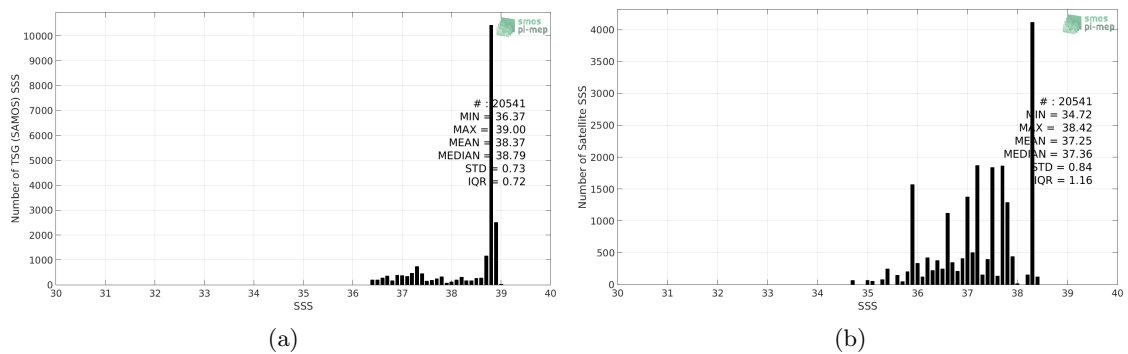
Figure 2: Histograms of SSS from TSG (SAMOS) (a) and SMOS SSS L3 v317 - 10 Days - 25 km (CATDS-CPDC) (b) considering all match-up pairs per bins of 0.1 over the Mediterranean Sea Pi-MEP region and for the full satellite product period.
