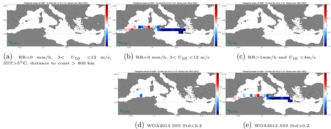
Figure 12: Temporal mean gridded over spatial boxes of size 1^{\circ}\times 1^{\circ} of \Delta\text{SSS} (SMOS L3 v317 - 10 Days - 25 km (CATDS-CPDC) - TSG-SAMOS) for 5 different subdatasets corresponding to: RR=0 mm/h, 3 < U_{10} < 12 m/s, SST > 5^{\circ}\text{C} , distance to coast > 800 km (a), RR=0 mm/h, 3 < U_{10} < 12 m/s (b), RR > 1 mm/h and U_{10} < 4 m/s (c), WOA2013 SSS Std < 0.2 (d), WOA2013 SSS Std > 0.2 (e).
