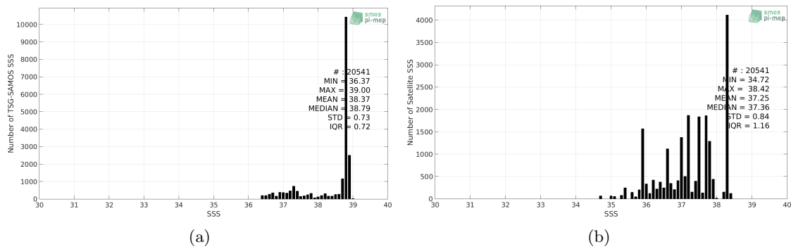
Figure 2: Histograms of SSS from TSG-SAMOS (a) and SMOS L3 v317 - 10 Days - 25 km (CATDS-CPDC) (b) considering all match-up pairs per bins of 0.1 over the Mediterranean Sea Pi-MEP region and for the full satellite product period.
