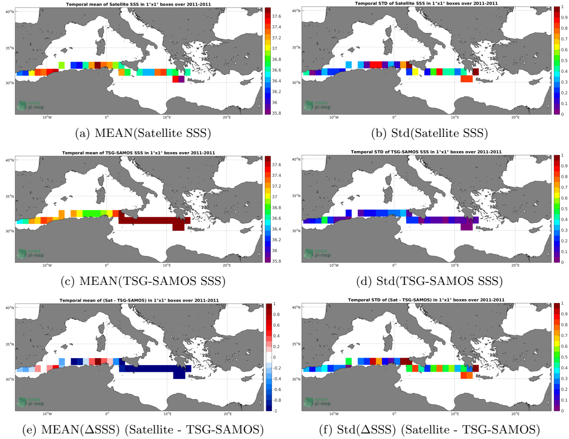
Figure 6: Temporal mean (left) and Std (right) of SSS from SMOS L3 v317 - 10 Days - 25 km (CATDS-CPDC) (top), TSG-SAMOS (middle), and of \Delta SSS (Satellite - TSG-SAMOS). Only match-up pairs are used to generate these maps.
