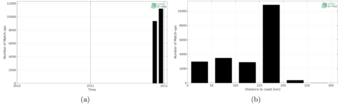
Figure 1: Number of match-ups between TSG-SAMOS and SMOS L3 v317 - 10 Days - 25 km (CATDS-CPDC) SSS as a function of time (a) and as function of the distance to coast (b) over the Mediterranean Sea Pi-MEP region and for the full satellite product period.
