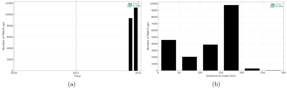
Figure 1: Number of match-ups between TSG-SAMOS and SMOS-L3-CATDS-CPDC-V317-10DAYS-25KM SSS as a function of time (a) and as function of the distance to coast (b) over the Mediterranean Sea Pi-MEP region and for the full satellite product period.
