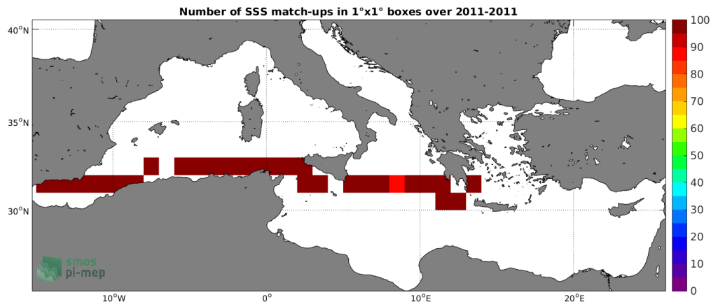
Figure 4: Number of SSS match-ups between TSG-SAMOS SSS and the SMOS-L3-CATDS-CPDC-V317-10DAYS-25KM SSS product for the Mediterranean Sea Pi-MEP region over 1^\circ \times 1^\circ boxes and for the full satellite product period.
