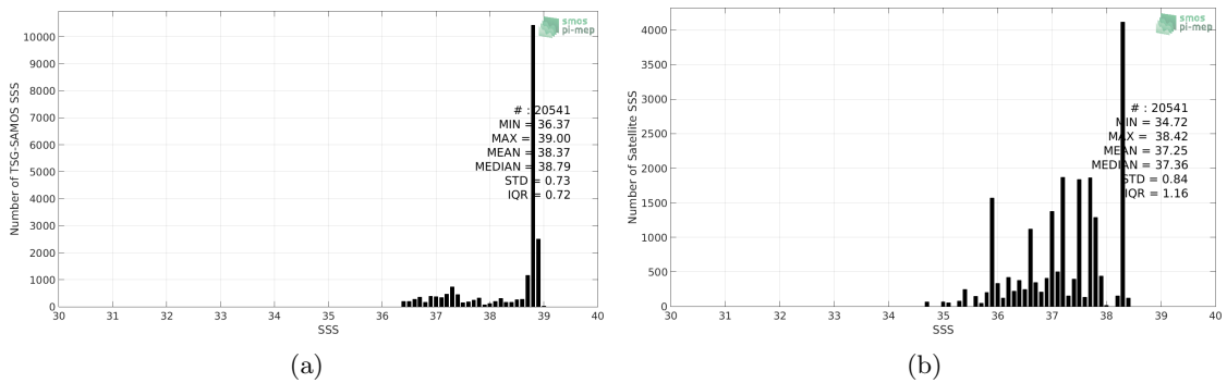
Figure 2: Histograms of SSS from TSG-SAMOS (a) and SMOS-L3-CATDS-CPDC-V317-10DAYS-25KM (b) considering all match-up pairs per bins of 0.1 over the Mediterranean Sea Pi-MEP region and for the full satellite product period.
