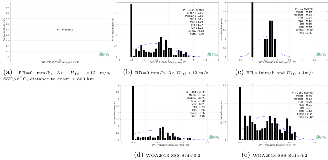
Figure 13: Normalized histogram of \Delta\text{SSS} (SMOS SSS L3 v317 - 10 Days - 25 km (CATDS-CPDC) - TSG (GOSUD-Sailing-ship)) for 5 different subdatasets corresponding to: RR=0 mm/h, 3 < U_{10} < 12 m/s, SST > 5^\circ\text{C} , distance to coast > 800 km (a), RR=0 mm/h, 3 < U_{10} < 12 m/s (b), RR > 1 mm/h and U_{10} < 4 m/s (c), WOA2013 SSS Std <0.2 (d), WOA2013 SSS Std >0.2 (e).
