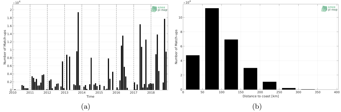
Figure 1: Number of match-ups between TSG-GOSUD-Research-vessel and SMOS L3 v317 - 10 Days - 25 km (CATDS-CPDC) SSS as a function of time (a) and as function of the distance to coast (b) over the Mediterranean Sea Pi-MEP region and for the full satellite product period.
