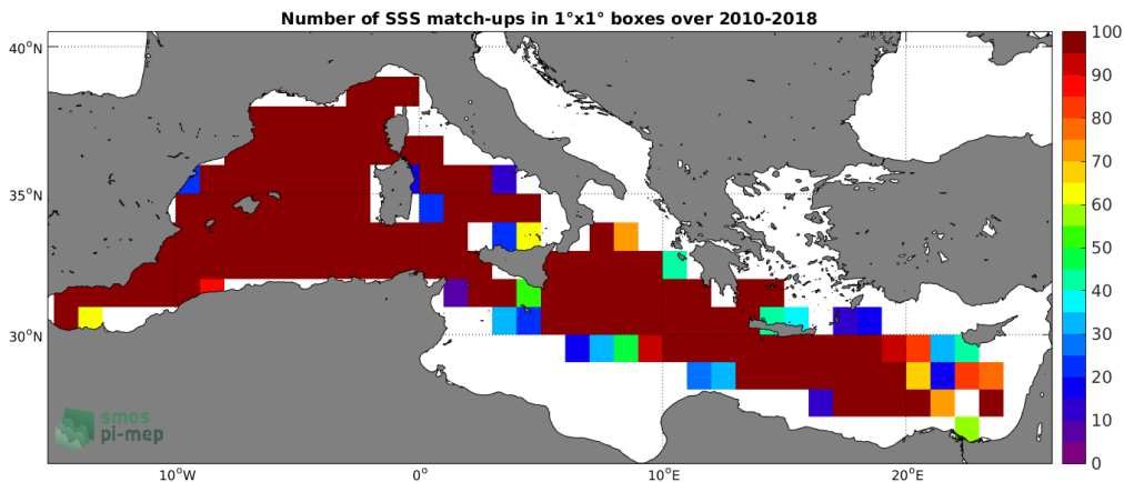
Figure 4: Number of SSS match-ups between TSG-GOSUD-Research-vessel SSS and the SMOS L3 v317 - 10 Days - 25 km (CATDS-CPDC) SSS product for the Mediterranean Sea Pi-MEP region over 1^\circ \times 1^\circ boxes and for the full satellite product period.
