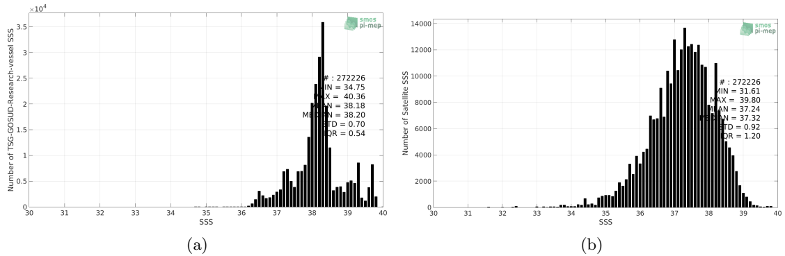
Figure 2: Histograms of SSS from TSG-GOSUD-Research-vessel (a) and SMOS L3 v317 - 10 Days - 25 km (CATDS-CPDC) (b) considering all match-up pairs per bins of 0.1 over the Mediterranean Sea Pi-MEP region and for the full satellite product period.
