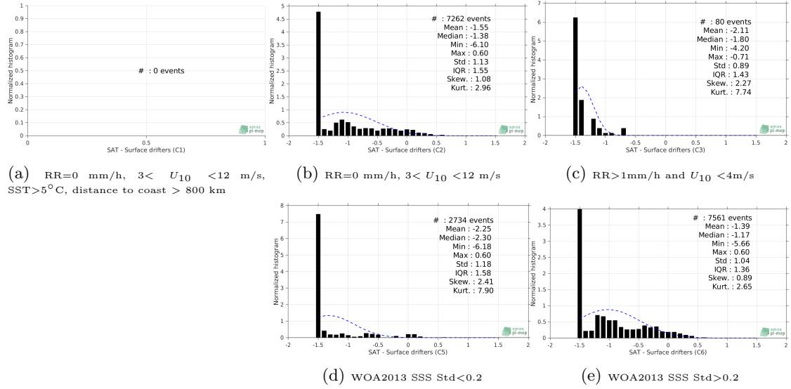
Figure 12: Normalized histogram of \Delta\text{SSS} (SMOS-L3-CATDS-CPDC-V317-10DAYS-25KM - Surface drifters) for 5 different subdatasets corresponding to: RR=0 mm/h, 3 < U_{10} < 12 m/s, SST > 5^{\circ}\text{C} , distance to coast > 800 km (a), RR=0 mm/h, 3 < U_{10} < 12 m/s (b), RR > 1\text{mm/h} and U_{10} < 4\text{m/s} (c), WOA2013 SSS Std < 0.2 (d), WOA2013 SSS Std > 0.2 (e).
