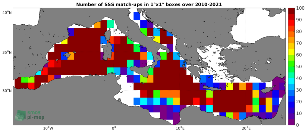
Figure 4: Number of SSS match-ups between Argo SSS and the SMOS SSS L3 v317 - 10 Days - 25 km (CATDS-CPDC) SSS product for the Mediterranean Sea Pi-MEP region over 1^\circ \times 1^\circ boxes and for the full satellite product period.
