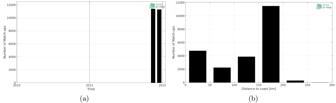
Figure 1: Number of match-ups between TSG-SAMOS and SMOS-L3-CATDS-CPDC-V3-MONTHLY-25KM SSS as a function of time (a) and as function of the distance to coast (b) over the Mediterranean Sea Pi-MEP region and for the full satellite product period.
