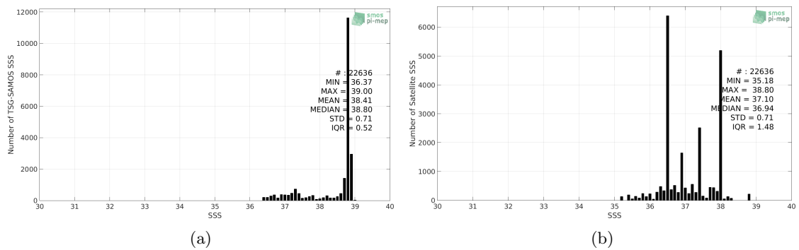
Figure 2: Histograms of SSS from TSG-SAMOS (a) and SMOS-L3-CATDS-CPDC-V3-MONTHLY-25KM (b) considering all match-up pairs per bins of 0.1 over the Mediterranean Sea Pi-MEP region and for the full satellite product period.
