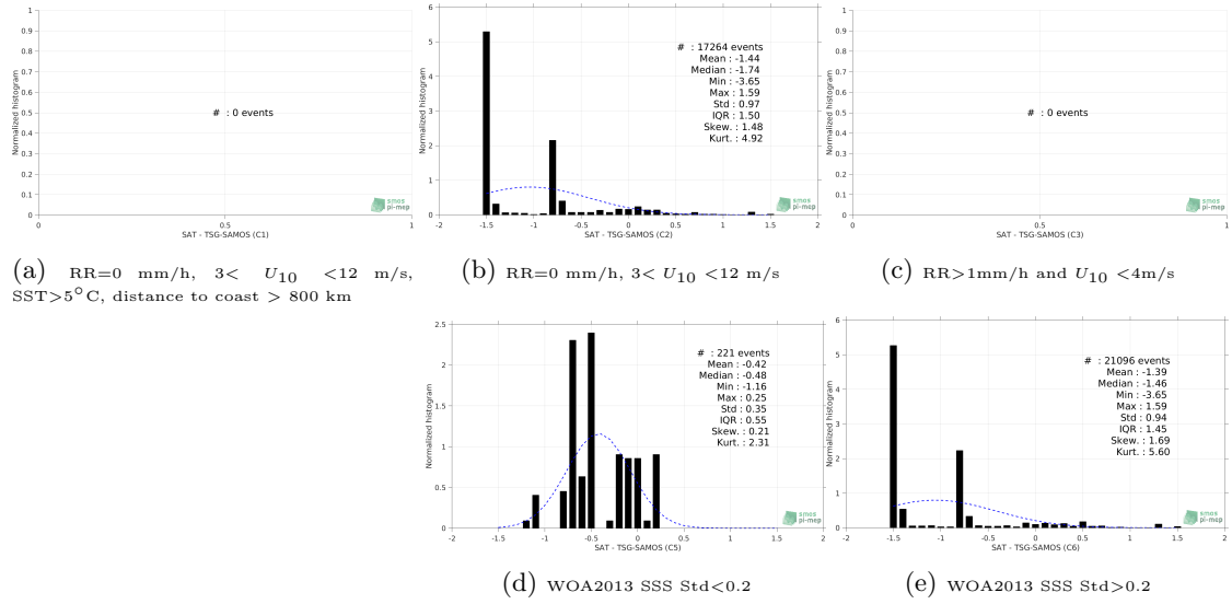
Figure 13: Normalized histogram of \Delta SSS (SMOS-L3-CATDS-CPDC-V3-MONTHLY-25KM - TSG-SAMOS) for 5 different subdatasets corresponding to: RR=0 mm/h, 3 < U_{10} < 12 m/s, SST > 5°C, distance to coast > 800 km (a), RR=0 mm/h, 3 < U_{10} < 12 m/s (b), RR > 1mm/h and U_{10} < 4 m/s (c), WOA2013 SSS Std < 0.2 (d), WOA2013 SSS Std > 0.2 (e).
