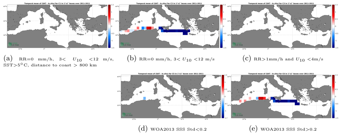
Figure 12: Temporal mean gridded over spatial boxes of size 1^\circ \times 1^\circ of \Delta SSS (SMOS-L3-CATDS-CPDC-V3-MONTHLY-25KM - TSG-SAMOS) for 5 different subdatasets corresponding to:RR=0 mm/h, 3 < U_{10} < 12 m/s, SST >5^\circ\text{C} , distance to coast > 800 km (a), RR=0 mm/h, 3 < U_{10} < 12 m/s (b), RR >1 mm/h and U_{10} < 4 m/s (c), WOA2013 SSS Std <0.2 (d), WOA2013 SSS Std >0.2 (e).
