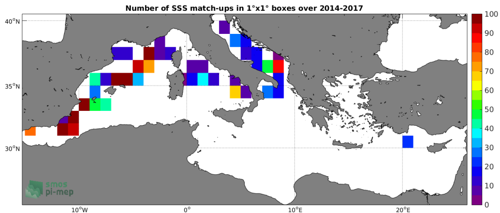
Figure 4: Number of SSS match-ups between TSG-GOSUD-Sailing-ship SSS and the SMOS-L3-CATDS-CPDC-V3-MONTHLY-25KM SSS product for the Mediterranean Sea Pi-MEP region over 1°x1° boxes and for the full satellite product period.
