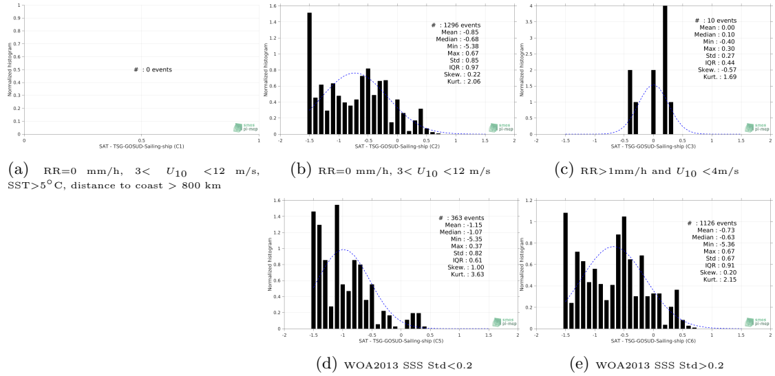
Figure 13: Normalized histogram of \Delta SSS (SMOS-L3-CATDS-CPDC-V3-MONTHLY-25KM - TSG-GOSUD-Sailing-ship) for 5 different subdatasets corresponding to: RR=0 mm/h, 3 < U_{10} < 12 m/s, SST > 5°C, distance to coast > 800 km (a), RR=0 mm/h, 3 < U_{10} < 12 m/s (b), RR > 1mm/h and U_{10} < 4 m/s (c), WOA2013 SSS Std < 0.2 (d), WOA2013 SSS Std > 0.2 (e).
