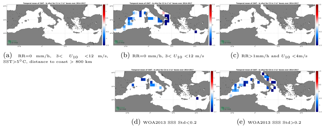
Figure 12: Temporal mean gridded over spatial boxes of size 1^\circ \times 1^\circ of \Delta SSS (SMOS-L3-CATDS-CPDC-V3-MONTHLY-25KM - TSG-GOSUD-Sailing-ship) for 5 different subdatasets corresponding to:RR=0 mm/h, 3 < U_{10} < 12 m/s, SST >5^\circ C, distance to coast > 800 km (a), RR=0 mm/h, 3 < U_{10} < 12 m/s (b), RR >1 mm/h and U_{10} < 4 m/s (c), WOA2013 SSS Std <0.2 (d), WOA2013 SSS Std >0.2 (e).
