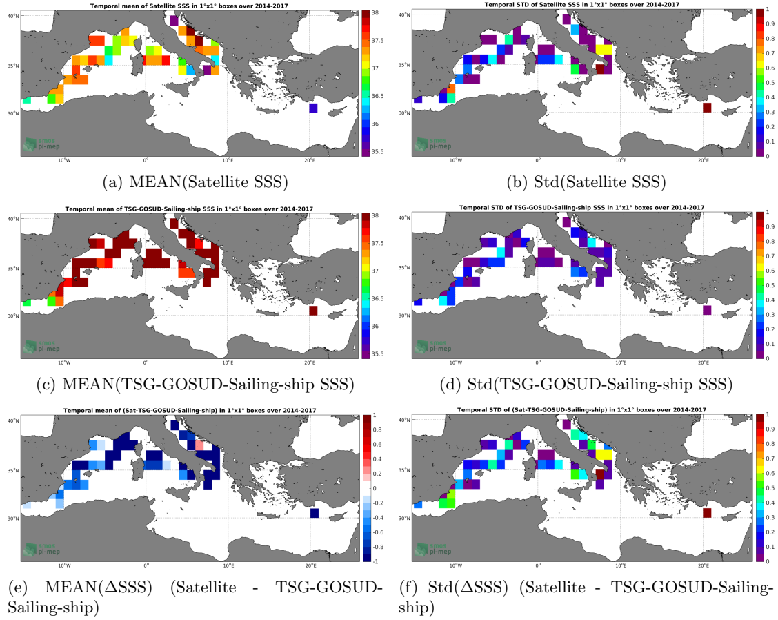
Figure 6: Temporal mean (left) and Std (right) of SSS from SMOS-L3-CATDS-CPDC-V3-MONTHLY-25KM (top), TSG-GOSUD-Sailing-ship (middle), and of \Delta SSS (Satellite - TSG-GOSUD-Sailing-ship). Only match-up pairs are used to generate these maps.
