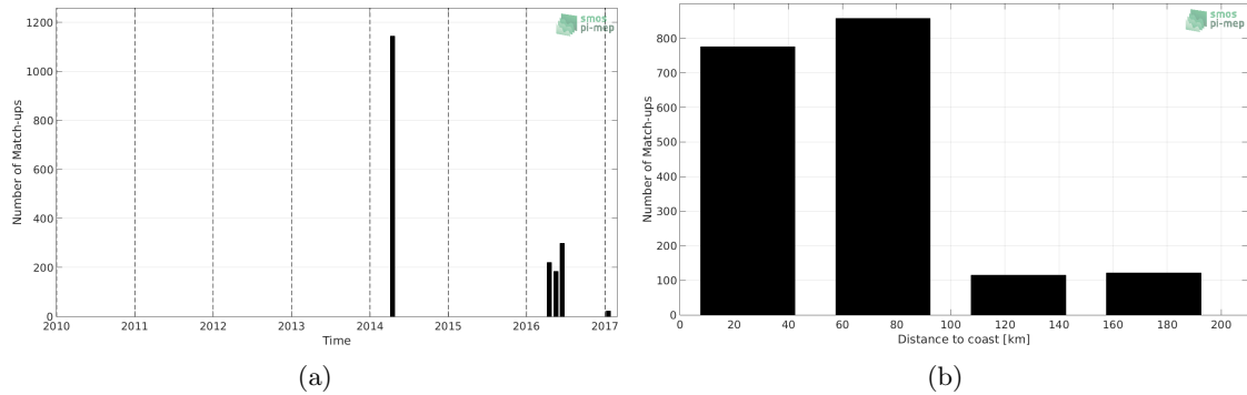
Figure 1: Number of match-ups between TSG-GOSUD-Sailing-ship and SMOS-L3-CATDS-CPDC-V3-MONTHLY-25KM SSS as a function of time (a) and as function of the distance to coast (b) over the Mediterranean Sea Pi-MEP region and for the full satellite product period.
