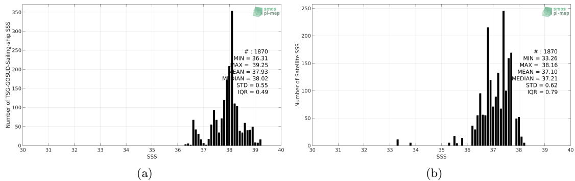
Figure 2: Histograms of SSS from TSG-GOSUD-Sailing-ship (a) and SMOS-L3-CATDS-CPDC-V3-MONTHLY-25KM (b) considering all match-up pairs per bins of 0.1 over the Mediterranean Sea Pi-MEP region and for the full satellite product period.
