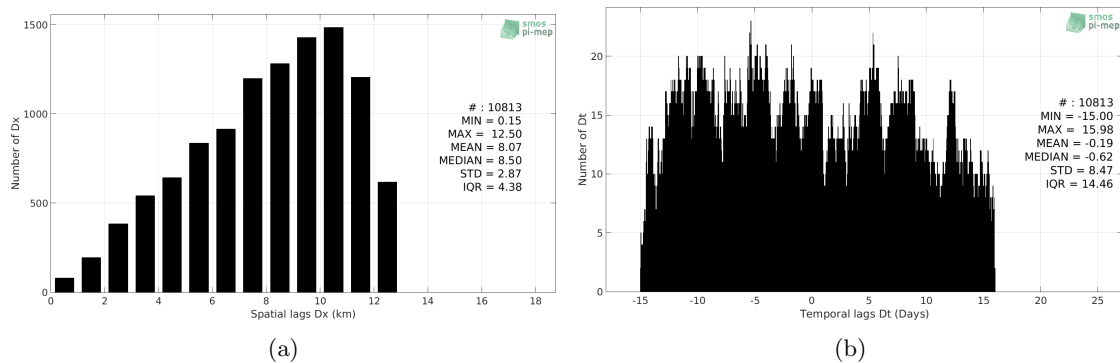
Figure 4: Histograms of the spatial (a) and temporal (b) lags between the time of the Surface drifters measurements and the date of the corresponding SMOS-L3-CATDS-CPDC-V3-MONTHLY-25KM SSS product.
