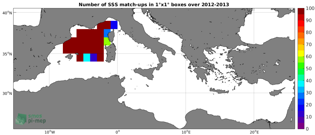
Figure 3: Number of SSS match-ups between Surface drifters SSS and the SMOS-L3-CATDS-CPDC-V3-MONTHLY-25KM SSS product for the Mediterranean Sea Pi-MEP region over 1^\circ \times 1^\circ boxes and for the full satellite product period.
