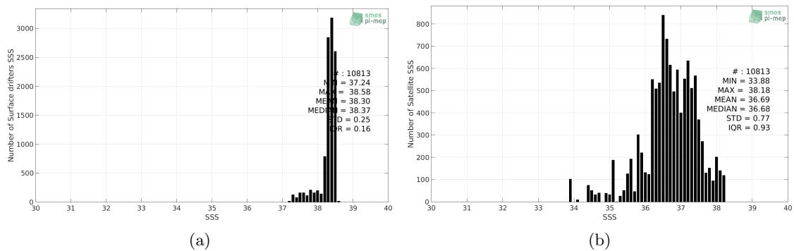
Figure 2: Histograms of SSS from Surface drifters (a) and SMOS-L3-CATDS-CPDC-V3-MONTHLY-25KM (b) considering all match-up pairs per bins of 0.1 over the Mediterranean Sea Pi-MEP region and for the full satellite product period.
