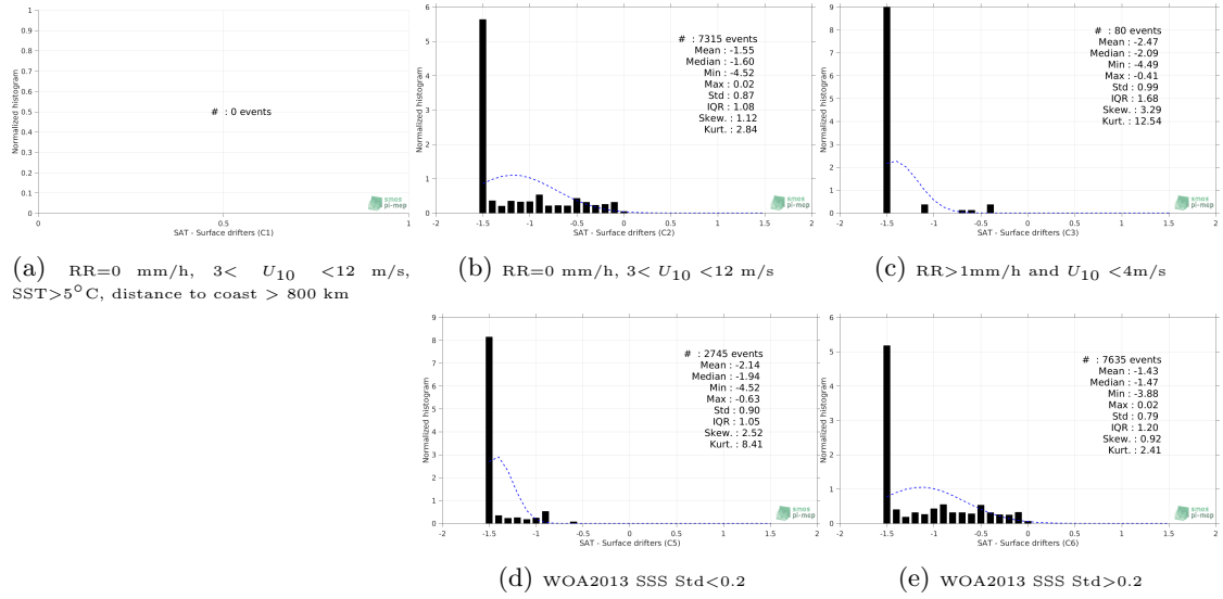
Figure 12: Normalized histogram of \Delta SSS (SMOS-L3-CATDS-CPDC-V3-MONTHLY-25KM - Surface drifters) for 5 different subdatasets corresponding to: RR=0 mm/h, 3 < U_{10} < 12 m/s, SST>5°C, distance to coast > 800 km (a), RR=0 mm/h, 3 < U_{10} < 12 m/s (b), RR>1mm/h and U_{10} < 4 m/s (c), WOA2013 SSS Std<0.2 (d), WOA2013 SSS Std>0.2 (e).
