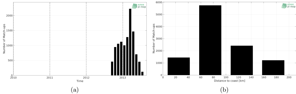
Figure 1: Number of match-ups between Surface drifters and SMOS-L3-CATDS-CPDC-V3-MONTHLY-25KM SSS as a function of time (a) and as function of the distance to coast (b) over the Mediterranean Sea Pi-MEP region and for the full satellite product period.
