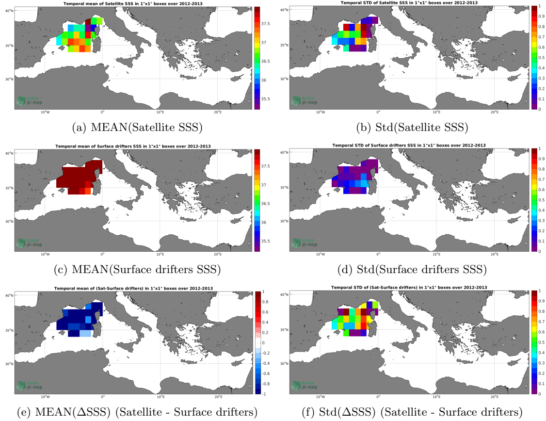
Figure 5: Temporal mean (left) and Std (right) of SSS from SMOS-L3-CATDS-CPDC-V3-MONTHLY-25KM (top), Surface drifters (middle), and of \Delta SSS (Satellite - Surface drifters). Only match-up pairs are used to generate these maps.
