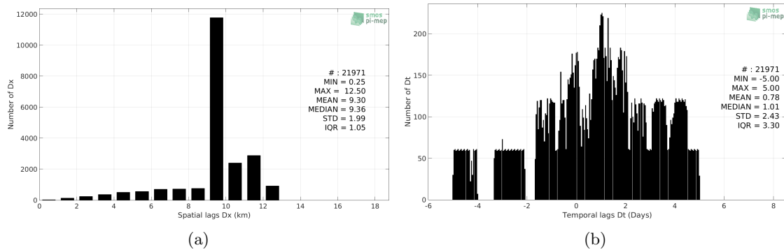
Figure 5: Histograms of the spatial (a) and temporal (b) lags between the time of the TSG-SAMOS measurements and the date of the corresponding SMOS-L3-CATDS-CPDC-V3-10DAYS-25KM SSS product.
