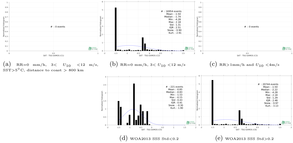
Figure 13: Normalized histogram of \Delta\text{SSS} (SMOS-L3-CATDS-CPDC-V3-10DAYS-25KM - TSG-SAMOS) for 5 different subdatasets corresponding to: RR=0 mm/h, 3 < U_{10} < 12 m/s, SST>5°C, distance to coast > 800 km (a), RR=0 mm/h, 3 < U_{10} < 12 m/s (b), RR>1mm/h and U_{10} < 4 m/s (c), WOA2013 SSS Std<0.2 (d), WOA2013 SSS Std>0.2 (e).
