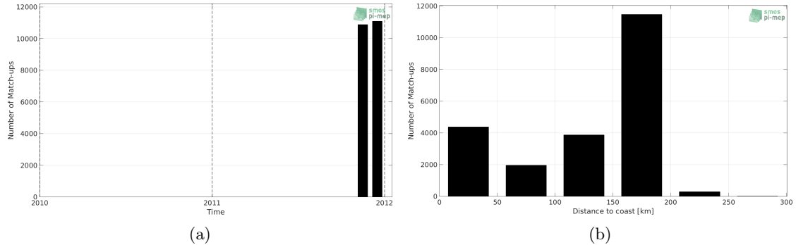
Figure 1: Number of match-ups between TSG-SAMOS and SMOS-L3-CATDS-CPDC-V3-10DAYS-25KM SSS as a function of time (a) and as function of the distance to coast (b) over the Mediterranean Sea Pi-MEP region and for the full satellite product period.
