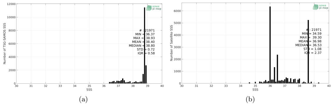
Figure 2: Histograms of SSS from TSG-SAMOS (a) and SMOS-L3-CATDS-CPDC-V3-10DAYS-25KM (b) considering all match-up pairs per bins of 0.1 over the Mediterranean Sea Pi-MEP region and for the full satellite product period.
