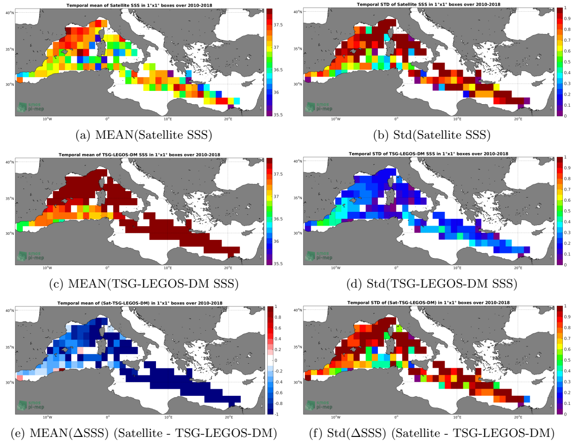
Figure 6: Temporal mean (left) and Std (right) of SSS from SMOS-L3-CATDS-CPDC-V3-10DAYS-25KM (top), TSG-LEGOS-DM (middle), and of \Delta SSS (Satellite - TSG-LEGOS-DM). Only match-up pairs are used to generate these maps.
