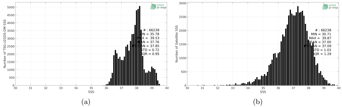
Figure 2: Histograms of SSS from TSG-LEGOS-DM (a) and SMOS-L3-CATDS-CPDC-V3-10DAYS-25KM (b) considering all match-up pairs per bins of 0.1 over the Mediterranean Sea Pi-MEP region and for the full satellite product period.
