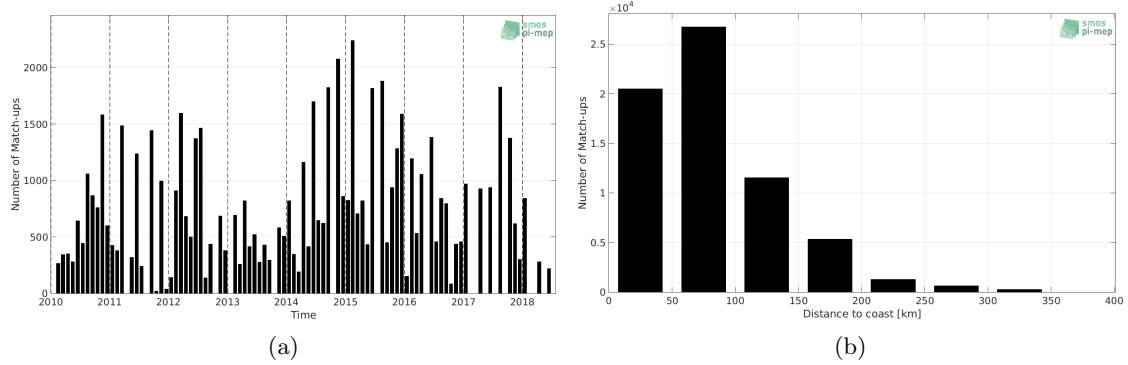
Figure 1: Number of match-ups between TSG-LEGOS-DM and SMOS-L3-CATDS-CPDC-V3-10DAYS-25KM SSS as a function of time (a) and as function of the distance to coast (b) over the Mediterranean Sea Pi-MEP region and for the full satellite product period.
