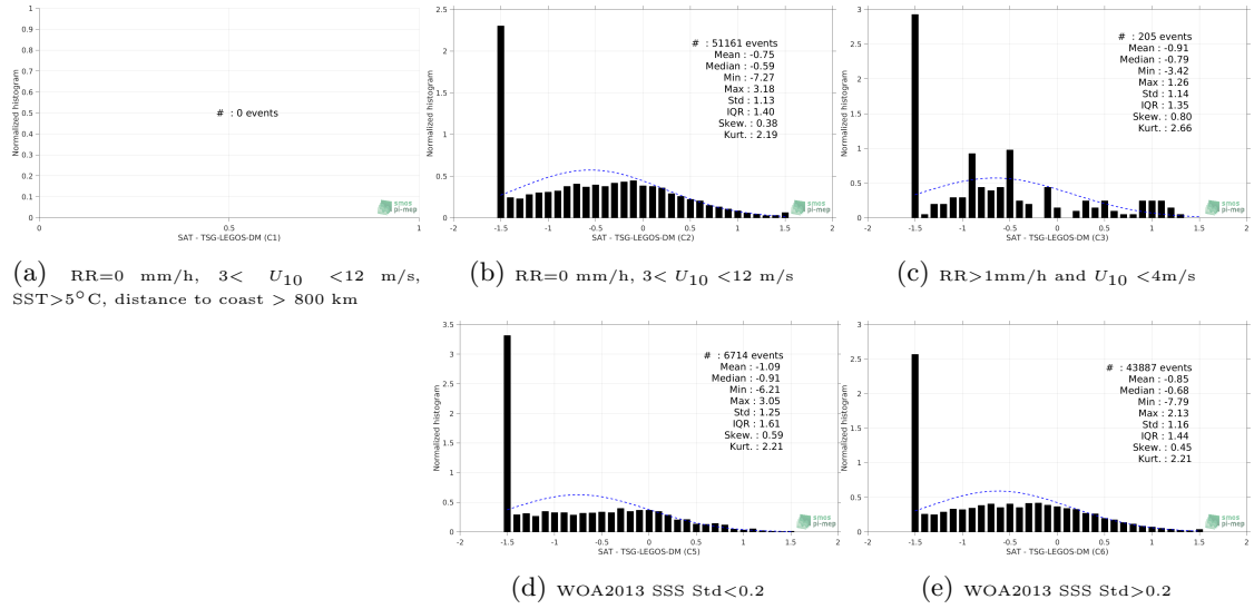
Figure 13: Normalized histogram of \Delta SSS (SMOS-L3-CATDS-CPDC-V3-10DAYS-25KM - TSG-LEGOS-DM) for 5 different subdatasets corresponding to: RR=0 mm/h, 3 < U_{10} < 12 m/s, SST > 5°C, distance to coast > 800 km (a), RR=0 mm/h, 3 < U_{10} < 12 m/s (b), RR > 1mm/h and U_{10} < 4 m/s (c), WOA2013 SSS Std < 0.2 (d), WOA2013 SSS Std > 0.2 (e).
