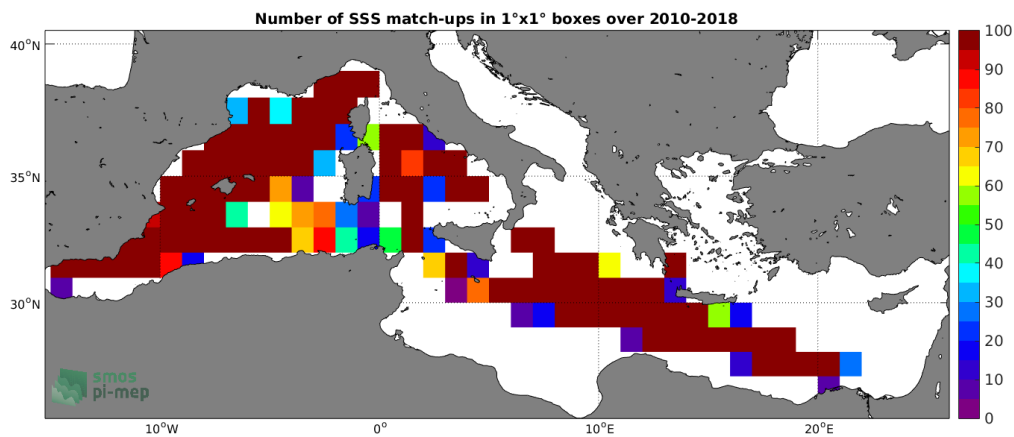
Figure 4: Number of SSS match-ups between TSG-LEGOS-DM SSS and the SMOS-L3-CATDS-CPDC-V3-10DAYS-25KM SSS product for the Mediterranean Sea Pi-MEP region over 1^\circ \times 1^\circ boxes and for the full satellite product period.
