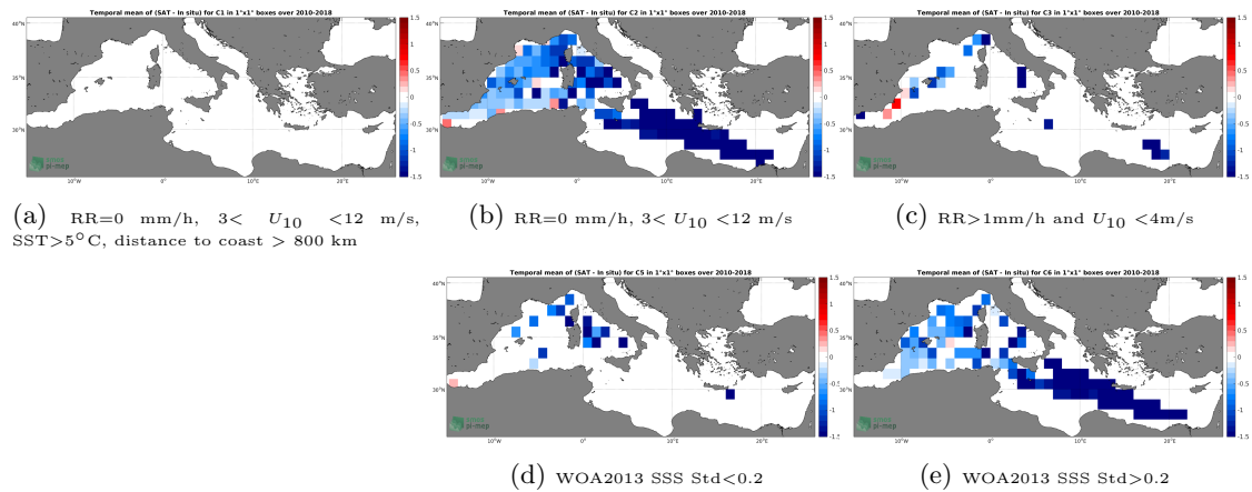
Figure 12: Temporal mean gridded over spatial boxes of size 1^\circ \times 1^\circ of \Delta SSS (SMOS-L3-CATDS-CPDC-V3-10DAYS-25KM - TSG-LEGOS-DM) for 5 different subdatasets corresponding to:RR=0 mm/h, 3 < U_{10} < 12 m/s, SST >5^\circ C, distance to coast > 800 km (a), RR=0 mm/h, 3 < U_{10} < 12 m/s (b), RR >1 mm/h and U_{10} < 4 m/s (c), WOA2013 SSS Std <0.2 (d), WOA2013 SSS Std >0.2 (e).
