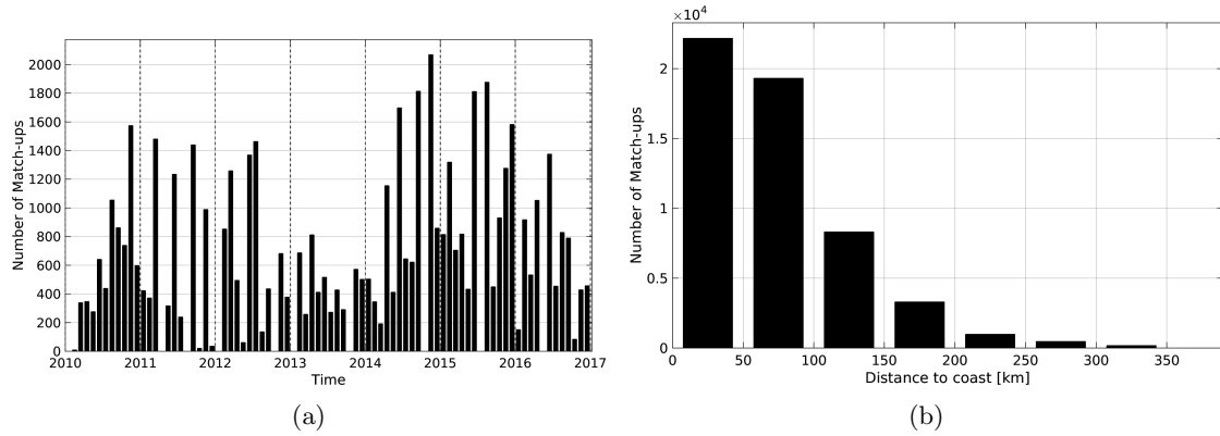
Figure 1: Number of match-ups between TSG-LEGOS-DM and SMOS-L3-CATDS-CPDC-V3-10DAYS-25KM SSS as a function of time (a) and as function of the distance to coast (b) over the Mediterranean Sea Pi-MEP region and for the full satellite product period.
