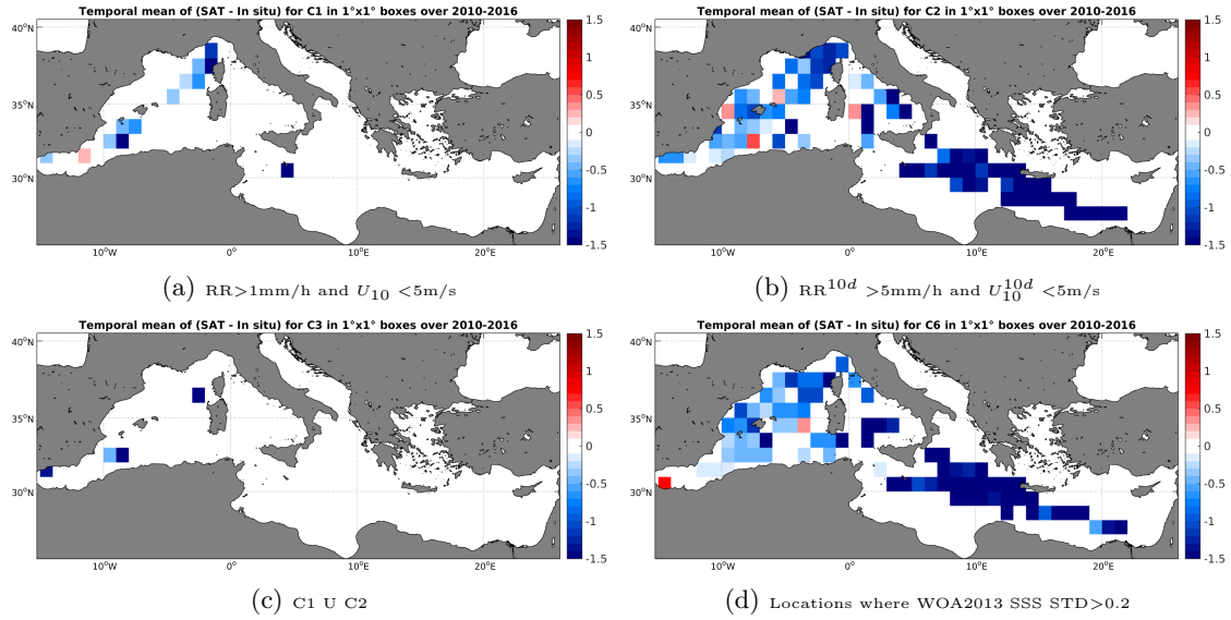
Figure 12: Temporal mean gridded over spatial boxes of size 1^\circ \times 1^\circ of \Delta SSS (SMOS-L3-CATDS-CPDC-V3-10DAYS-25KM - TSG-LEGOS-DM) for 4 different subdatasets corresponding to: RR > 1mm/h and U_{10} < 5m/s (a), RR^{10d} > 5mm/h and U_{10}^{10d} < 5m/s (b), C1 U C2 (c), Locations where WOA2013 SSS STD > 0.2 (d).
