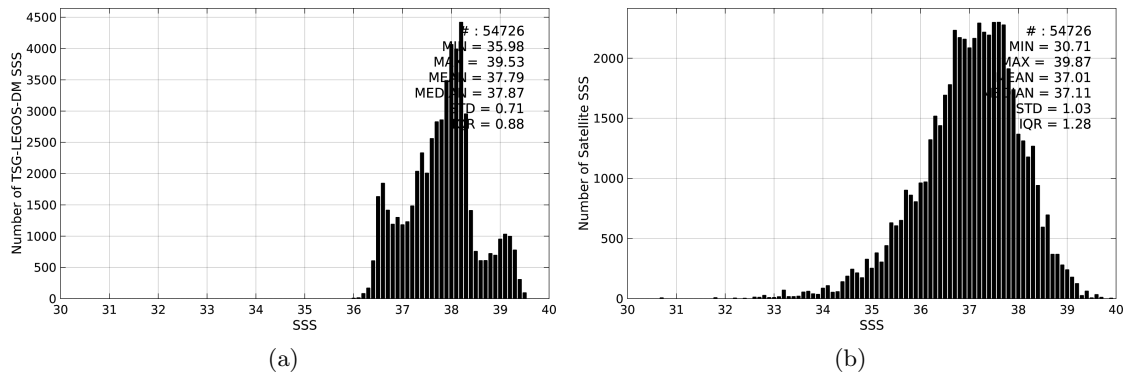
Figure 2: Histograms of SSS from TSG-LEGOS-DM (a) and SMOS-L3-CATDS-CPDC-V3-10DAYS-25KM (b) considering all match-up pairs per bins of 0.1 over the Mediterranean Sea Pi-MEP region and for the full satellite product period.
