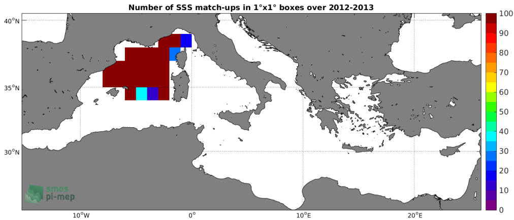
Figure 3: Number of SSS match-ups between Surface drifters SSS and the SMOS-L3-CATDS-CPDC-V3-10DAYS-25KM SSS product for the Mediterranean Sea Pi-MEP region over 1^\circ \times 1^\circ boxes and for the full satellite product period.
