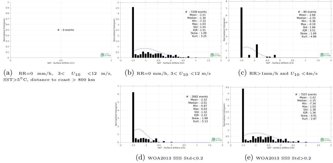
Figure 12: Normalized histogram of \Delta SSS (SMOS-L3-CATDS-CPDC-V3-10DAYS-25KM - Surface drifters) for 5 different subdatasets corresponding to: RR=0 mm/h, 3 < U_{10} < 12 m/s, SST > 5°C, distance to coast > 800 km (a), RR=0 mm/h, 3 < U_{10} < 12 m/s (b), RR > 1mm/h and U_{10} < 4 m/s (c), WOA2013 SSS Std < 0.2 (d), WOA2013 SSS Std > 0.2 (e).
