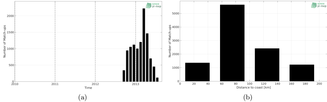
Figure 1: Number of match-ups between Surface drifters and SMOS-L3-CATDS-CPDC-V3-10DAYS-25KM SSS as a function of time (a) and as function of the distance to coast (b) over the Mediterranean Sea Pi-MEP region and for the full satellite product period.
