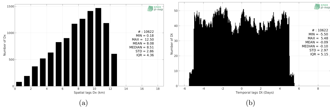
Figure 4: Histograms of the spatial (a) and temporal (b) lags between the time of the Surface drifters measurements and the date of the corresponding SMOS-L3-CATDS-CPDC-V3-10DAYS-25KM SSS product.
