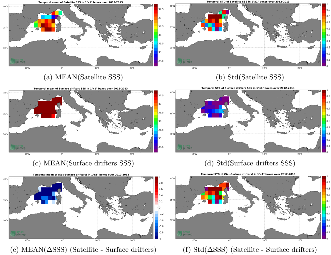
Figure 5: Temporal mean (left) and Std (right) of SSS from SMOS-L3-CATDS-CPDC-V3-10DAYS-25KM (top), Surface drifters (middle), and of \Delta SSS (Satellite - Surface drifters). Only match-up pairs are used to generate these maps.
