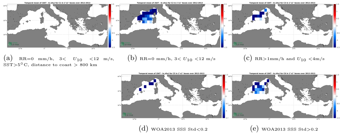
Figure 11: Temporal mean gridded over spatial boxes of size 1^\circ \times 1^\circ of \Delta SSS (SMOS-L3-CATDS-CPDC-V3-10DAYS-25KM - Surface drifters) for 5 different subdatasets corresponding to:RR=0 mm/h, 3 < U_{10} < 12 m/s, SST >5^\circ C, distance to coast > 800 km (a), RR=0 mm/h, 3 < U_{10} < 12 m/s (b), RR >1 mm/h and U_{10} < 4 m/s (c), WOA2013 SSS Std <0.2 (d), WOA2013 SSS Std >0.2 (e).
