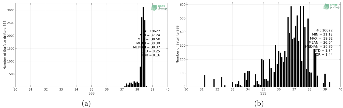
Figure 2: Histograms of SSS from Surface drifters (a) and SMOS-L3-CATDS-CPDC-V3-10DAYS-25KM (b) considering all match-up pairs per bins of 0.1 over the Mediterranean Sea Pi-MEP region and for the full satellite product period.
