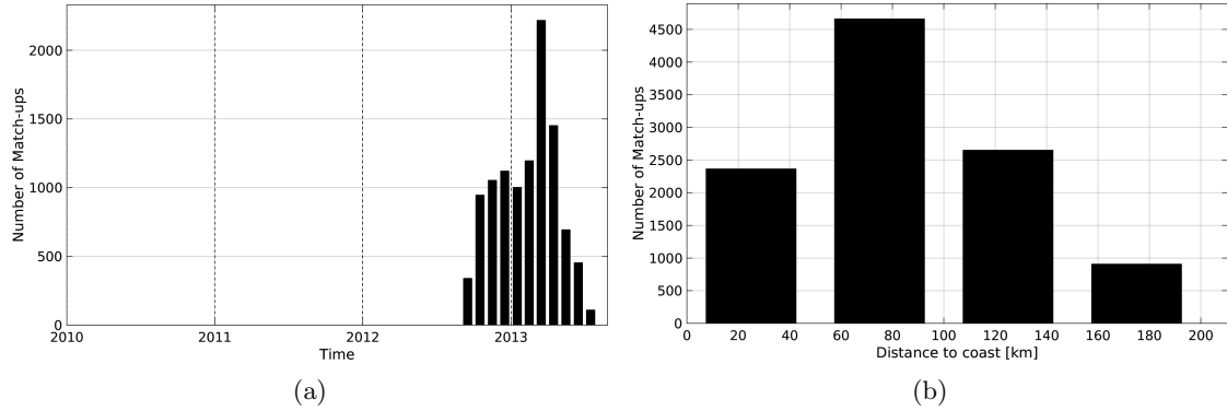
Figure 1: Number of match-ups between Surface drifters and SMOS-L3-CATDS-CPDC-V3-10DAYS-25KM SSS as a function of time (a) and as function of the distance to coast (b) over the Mediterranean Sea Pi-MEP region and for the full satellite product period.
