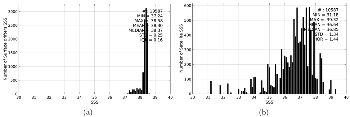
Figure 2: Histograms of SSS from Surface drifters (a) and SMOS-L3-CATDS-CPDC-V3-10DAYS-25KM (b) considering all match-up pairs per bins of 0.1 over the Mediterranean Sea Pi-MEP region and for the full satellite product period.
